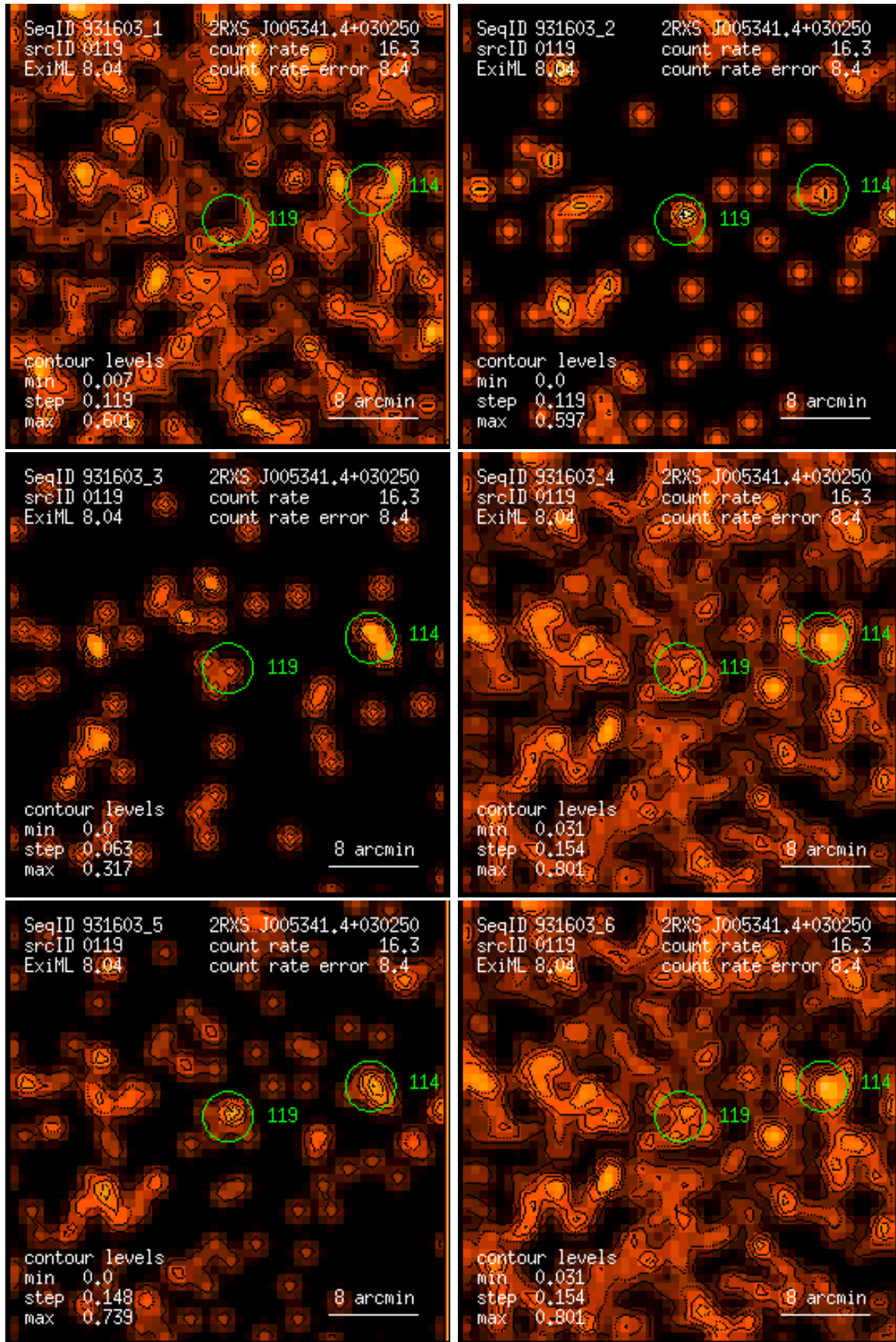
Figure 119: RASS 931603: detection 0119: band rate images, Gaussian filter: (1) PSPC channels 11 – 41, (2) 52 – 90, (3) 91 – 201, (4) 11 – 235, (5) 52 – 201, (6) 11 – 201. Broad band rates in counts/ks. Band rate contour levels in counts/ks/arcmin 2 .
