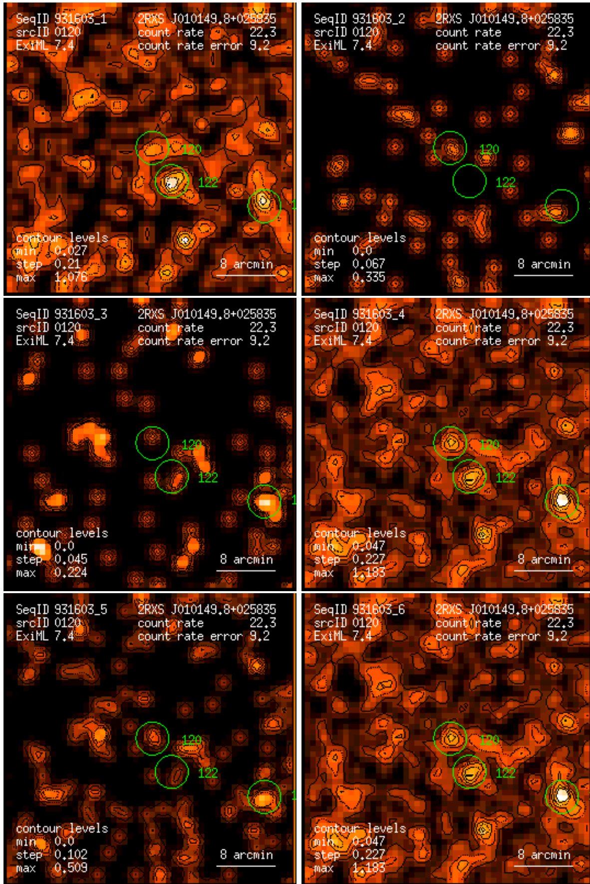
Figure 120: RASS 931603: detection 0120: band rate images, Gaussian filter: (1) PSPC channels 11 – 41, (2) 52 – 90, (3) 91 – 201, (4) 11 – 235, (5) 52 – 201, (6) 11 – 201. Broad band rates in counts/ks. Band rate contour levels in counts/ks/arcmin 2 .
