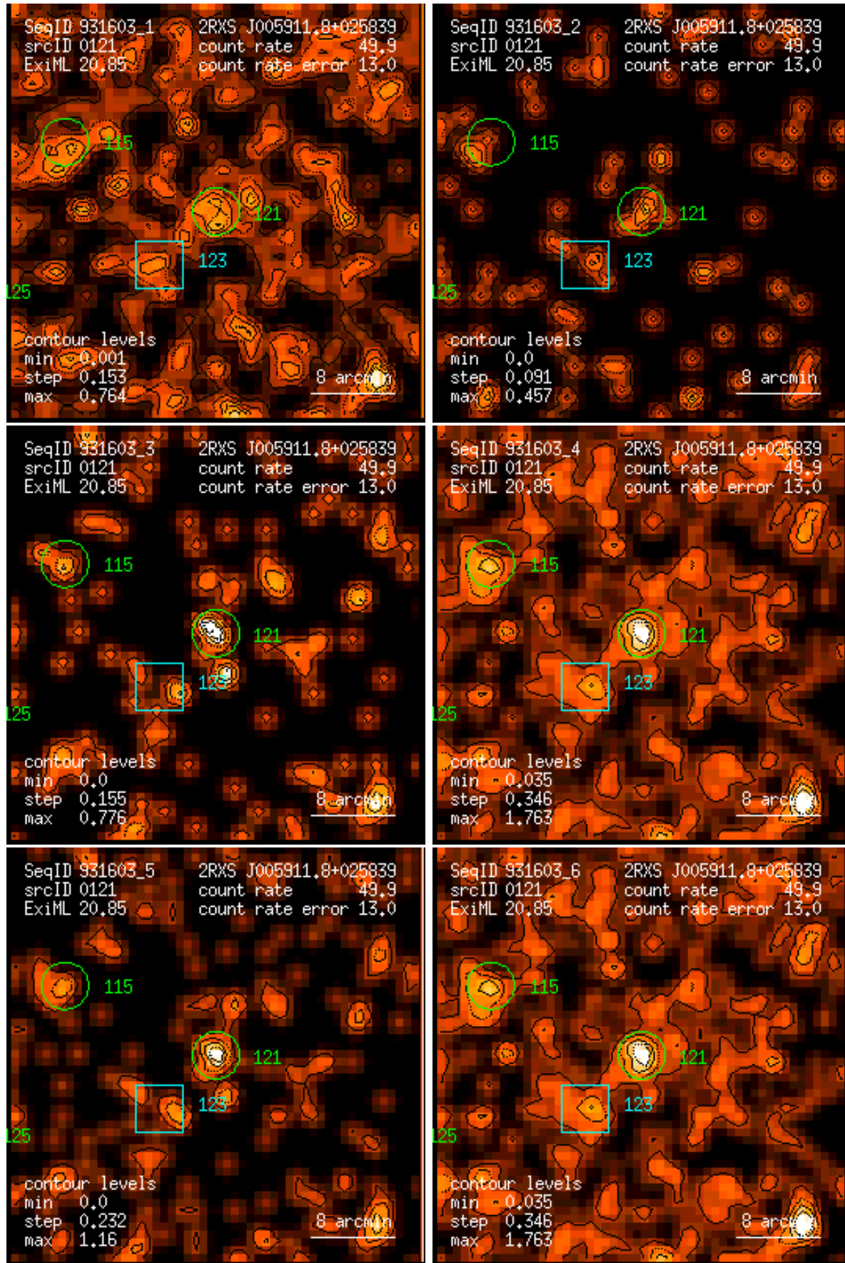
Figure 121: RASS 931603: detection 0121: band rate images, Gaussian filter: (1) PSPC channels 11 – 41, (2) 52 – 90, (3) 91 – 201, (4) 11 – 235, (5) 52 – 201, (6) 11 – 201. Broad band rates in counts/ks. Band rate contour levels in counts/ks/arcmin 2 .
