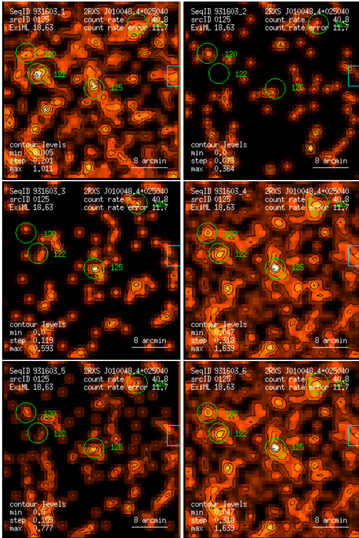
Figure 125: RASS 931603: detection 0125: band rate images, Gaussian filter: (1) PSPC channels 11 – 41, (2) 52 – 90, (3) 91 – 201, (4) 11 – 235, (5) 52 – 201, (6) 11 – 201. Broad band rates in counts/ks. Band rate contour levels in counts/ks/arcmin 2 .
