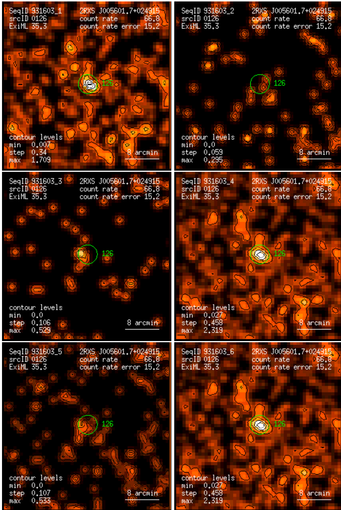
Figure 126: RASS 931603: detection 0126: band rate images, Gaussian filter: (1) PSPC channels 11 – 41, (2) 52 – 90, (3) 91 – 201, (4) 11 – 235, (5) 52 – 201, (6) 11 – 201. Broad band rates in counts/ks. Band rate contour levels in counts/ks/arcmin 2 .
