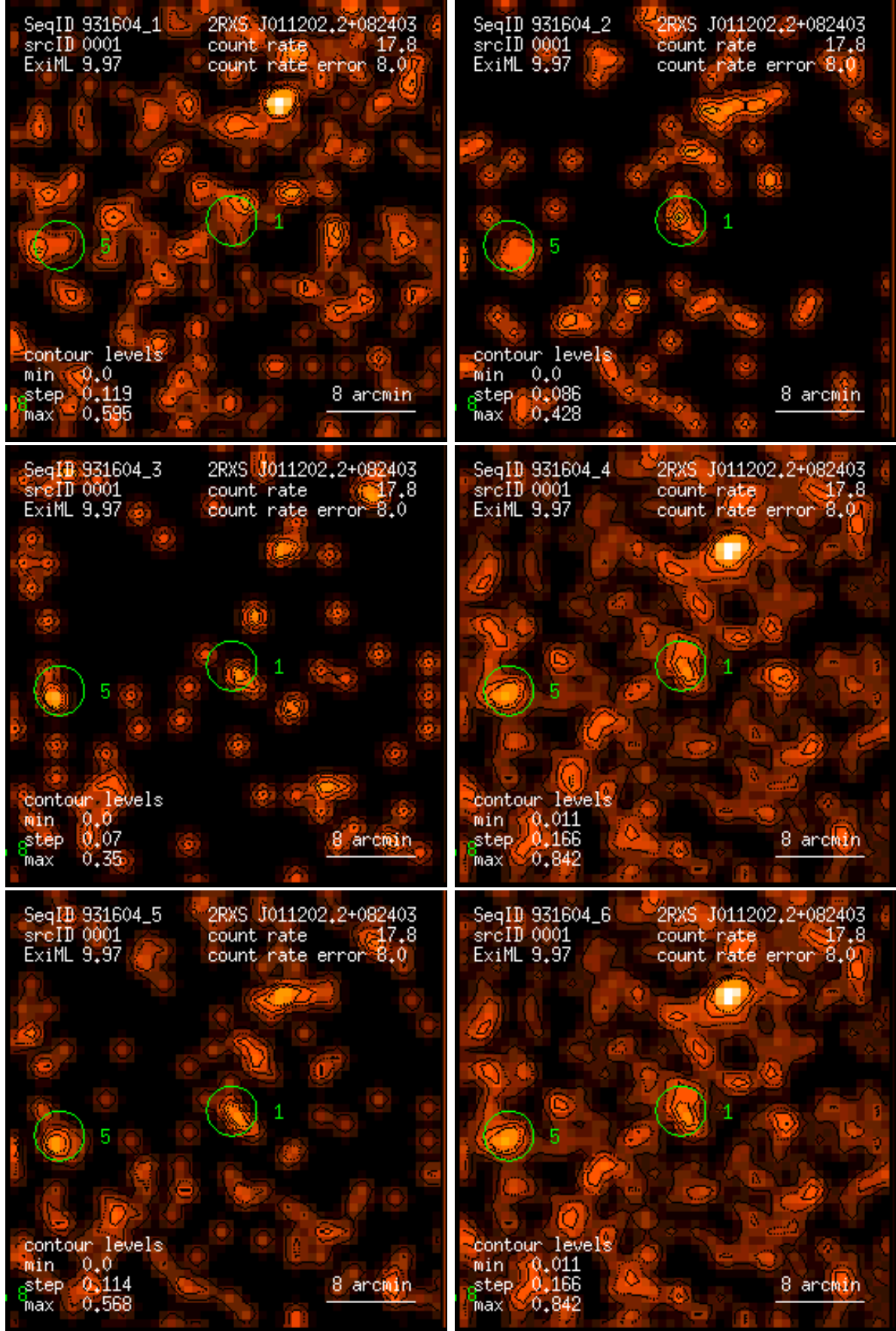
Figure 1: RASS 931604: detection 0001: band rate images, Gaussian filter: (1) PSPC channels 11 – 41, (2) 52 – 90, (3) 91 – 201, (4) 11 – 235, (5) 52 – 201, (6) 11 – 201. Broad band rates in counts/ks. Band rate contour levels in counts/ks/arcmin 2 .
