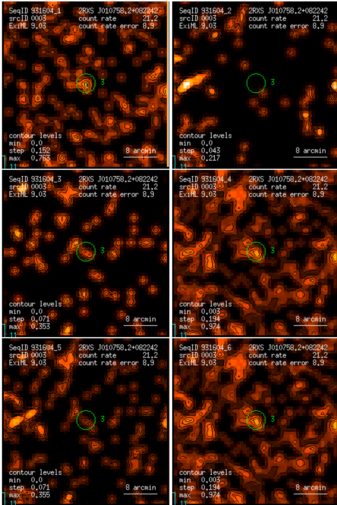
Figure 3: RASS 931604: detection 0003: band rate images, Gaussian filter: (1) PSPC channels 11 – 41, (2) 52 – 90, (3) 91 – 201, (4) 11 – 235, (5) 52 – 201, (6) 11 – 201. Broad band rates in counts/ks. Band rate contour levels in counts/ks/arcmin 2 .
