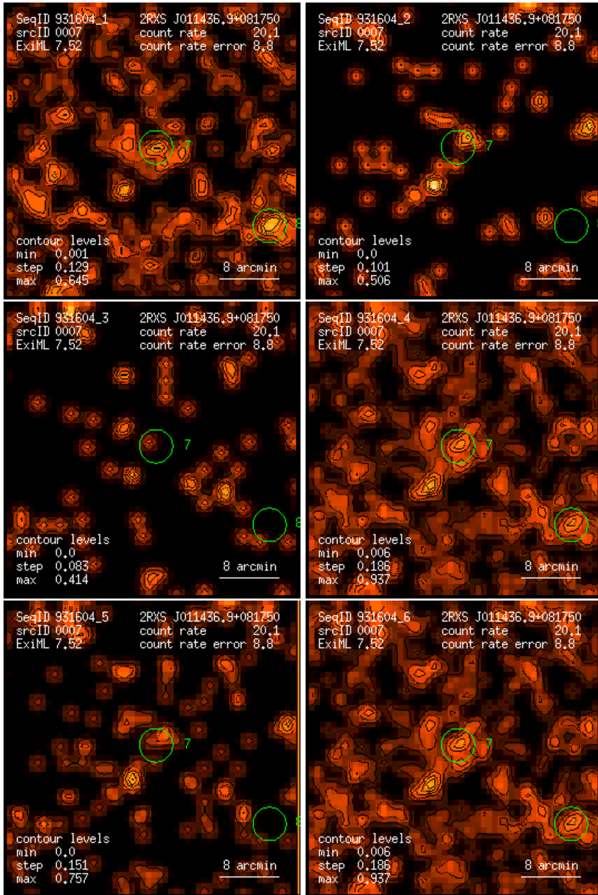
Figure 7: RASS 931604: detection 0007: band rate images, Gaussian filter: (1) PSPC channels 11 – 41, (2) 52 – 90, (3) 91 – 201, (4) 11 – 235, (5) 52 – 201, (6) 11 – 201. Broad band rates in counts/ks. Band rate contour levels in counts/ks/arcmin 2 .
