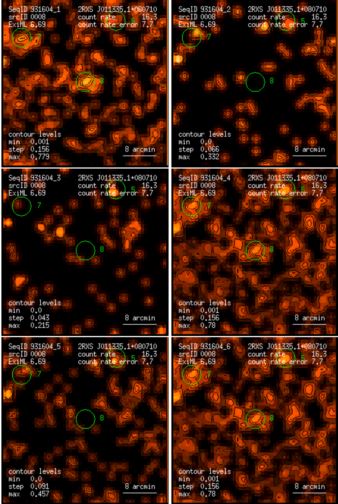
Figure 8: RASS 931604: detection 0008: band rate images, Gaussian filter: (1) PSPC channels 11 – 41, (2) 52 – 90, (3) 91 – 201, (4) 11 – 235, (5) 52 – 201, (6) 11 – 201. Broad band rates in counts/ks. Band rate contour levels in counts/ks/arcmin 2 .
