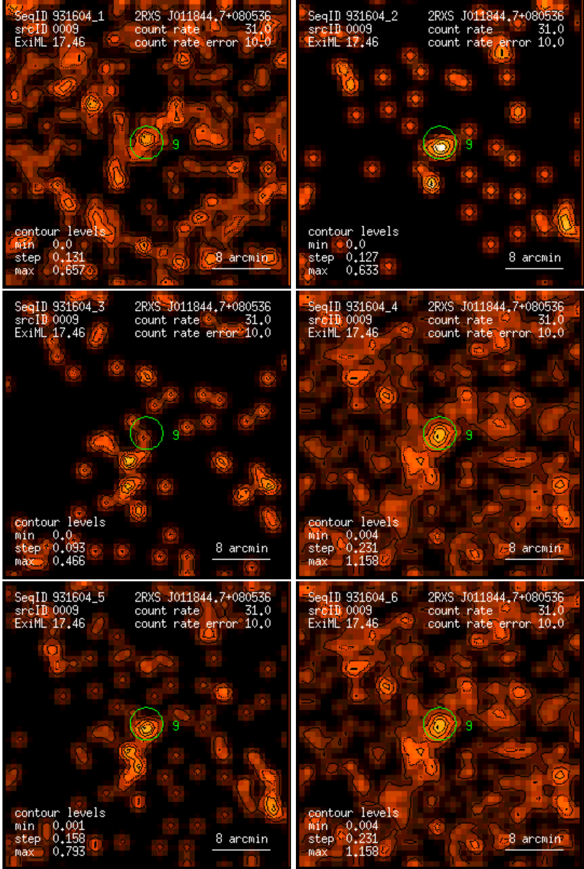
Figure 9: RASS 931604: detection 0009: band rate images, Gaussian filter: (1) PSPC channels 11 – 41, (2) 52 – 90, (3) 91 – 201, (4) 11 – 235, (5) 52 – 201, (6) 11 – 201. Broad band rates in counts/ks. Band rate contour levels in counts/ks/arcmin 2 .
