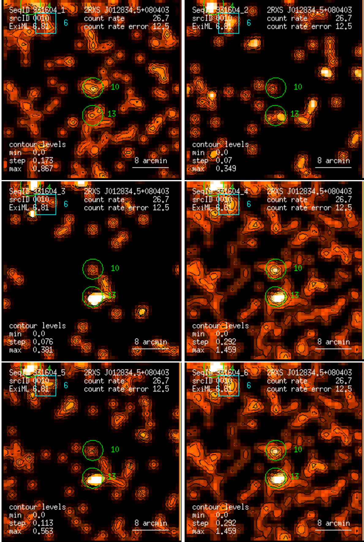
Figure 10: RASS 931604: detection 0010: band rate images, Gaussian filter: (1) PSPC channels 11 – 41, (2) 52 – 90, (3) 91 – 201, (4) 11 – 235, (5) 52 – 201, (6) 11 – 201. Broad band rates in counts/ks. Band rate contour levels in counts/ks/arcmin 2 .
