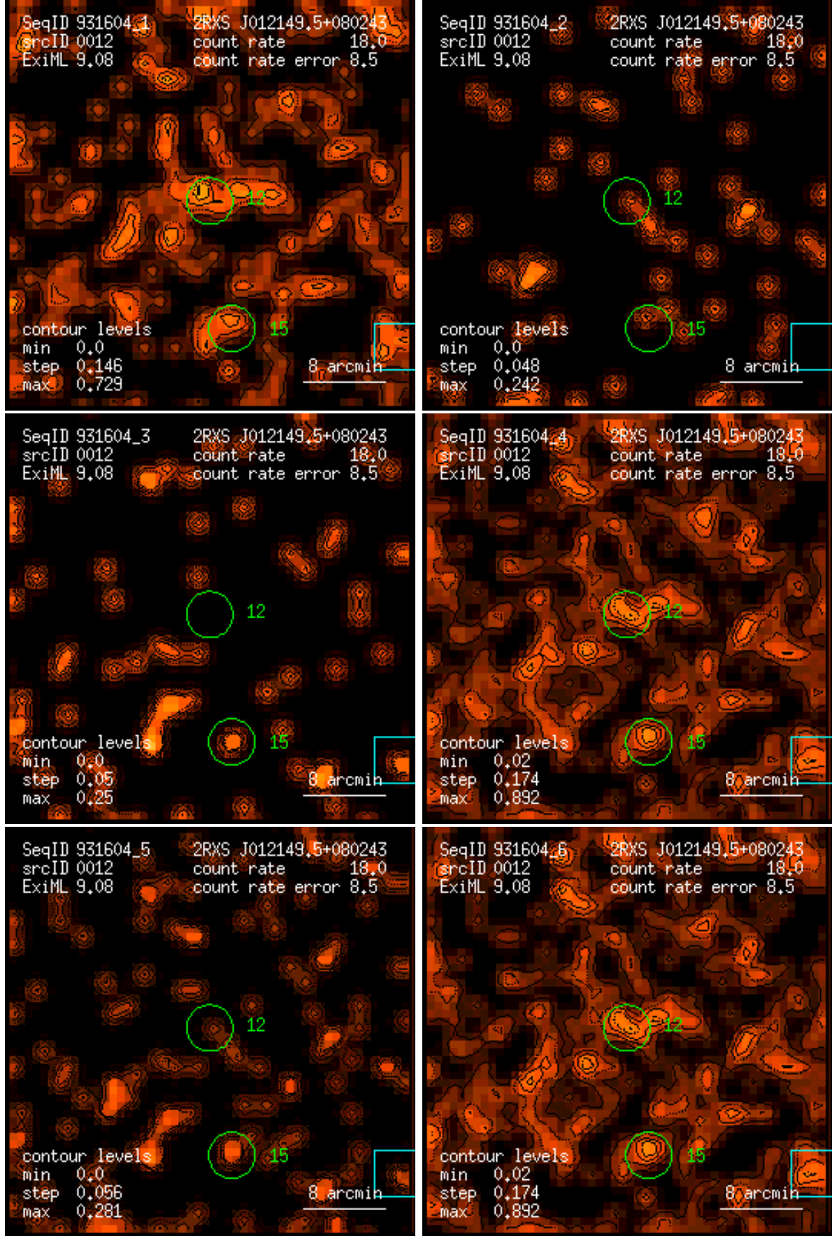
Figure 12: RASS 931604: detection 0012: band rate images, Gaussian filter: (1) PSPC channels 11 – 41, (2) 52 – 90, (3) 91 – 201, (4) 11 – 235, (5) 52 – 201, (6) 11 – 201. Broad band rates in counts/ks. Band rate contour levels in counts/ks/arcmin 2 .
