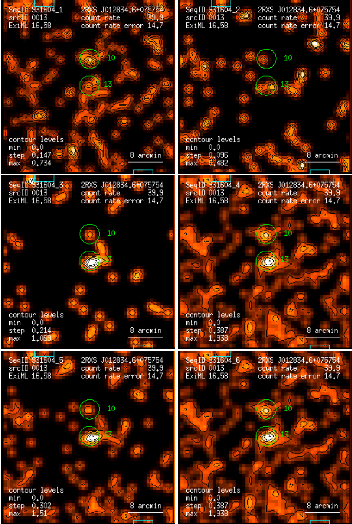
Figure 13: RASS 931604: detection 0013: band rate images, Gaussian filter: (1) PSPC channels 11 – 41, (2) 52 – 90, (3) 91 – 201, (4) 11 – 235, (5) 52 – 201, (6) 11 – 201. Broad band rates in counts/ks. Band rate contour levels in counts/ks/arcmin 2 .
