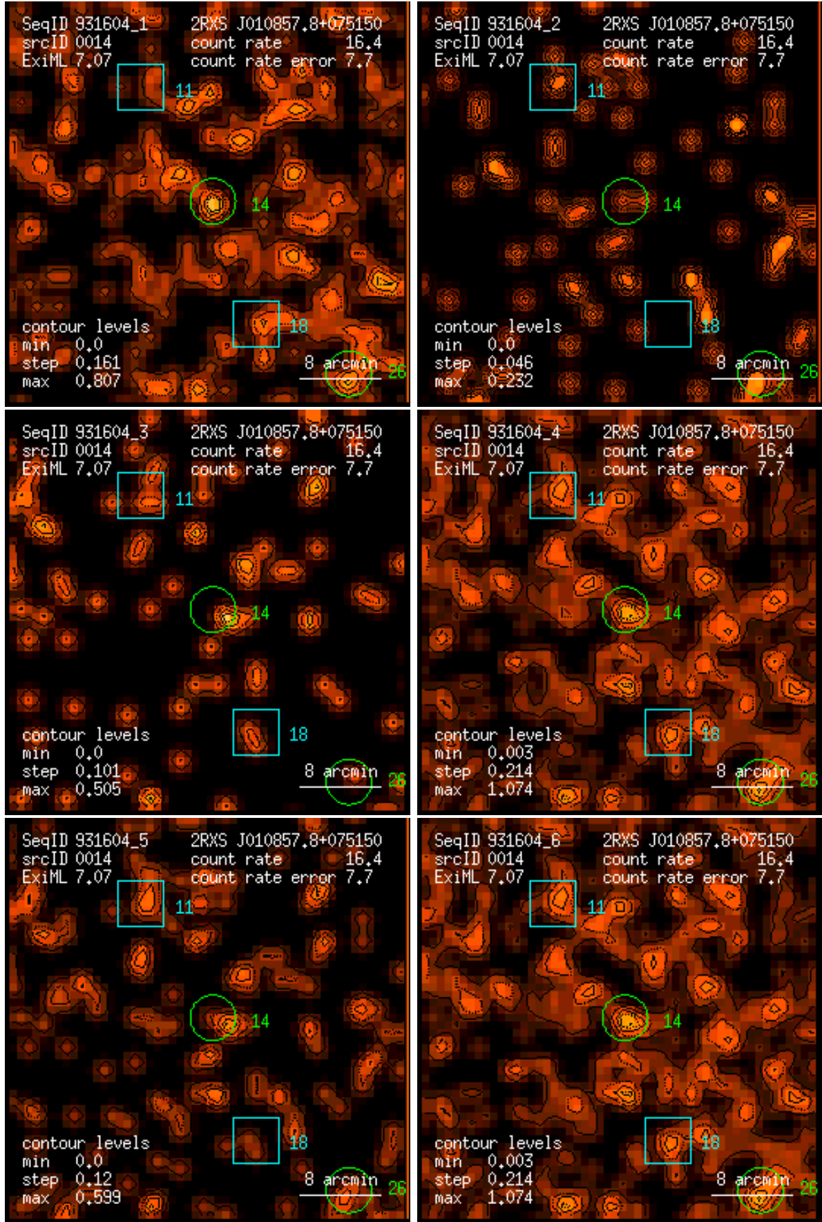
Figure 14: RASS 931604: detection 0014: band rate images, Gaussian filter: (1) PSPC channels 11 – 41, (2) 52 – 90, (3) 91 – 201, (4) 11 – 235, (5) 52 – 201, (6) 11 – 201. Broad band rates in counts/ks. Band rate contour levels in counts/ks/arcmin 2 .
