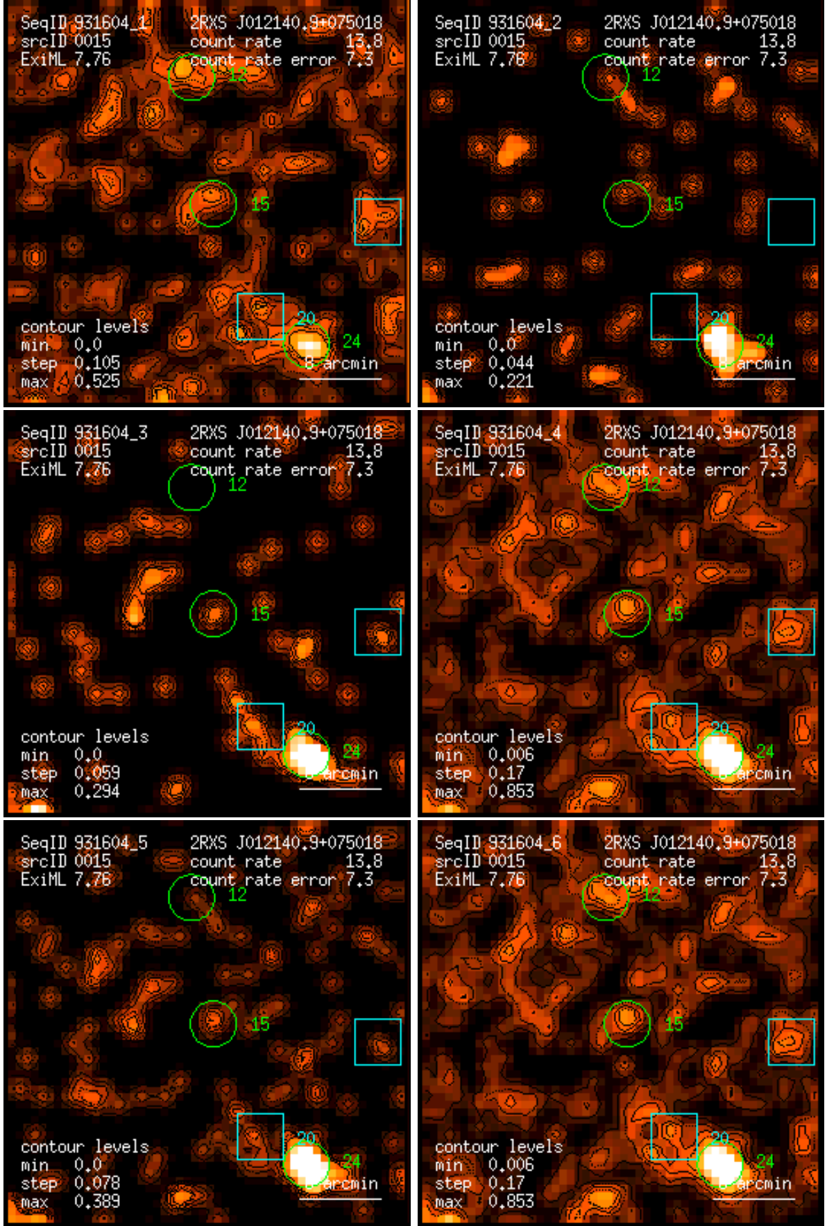
Figure 15: RASS 931604: detection 0015: band rate images, Gaussian filter: (1) PSPC channels 11 – 41, (2) 52 – 90, (3) 91 – 201, (4) 11 – 235, (5) 52 – 201, (6) 11 – 201. Broad band rates in counts/ks. Band rate contour levels in counts/ks/arcmin 2 .
