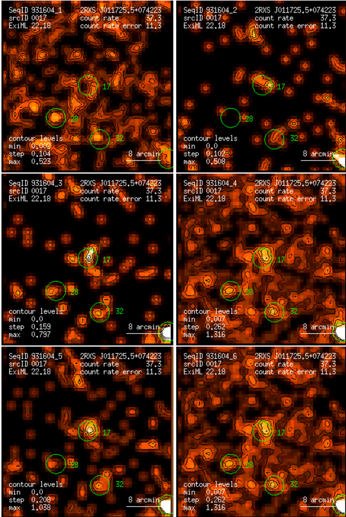
Figure 17: RASS 931604: detection 0017: band rate images, Gaussian filter: (1) PSC channels 11 – 41, (2) 52 – 90, (3) 91 – 201, (4) 11 – 235, (5) 52 – 201, (6) 11 – 201. Broad band rates in counts/ks. Band rate contour levels in counts/ks/arcmin 2 .
