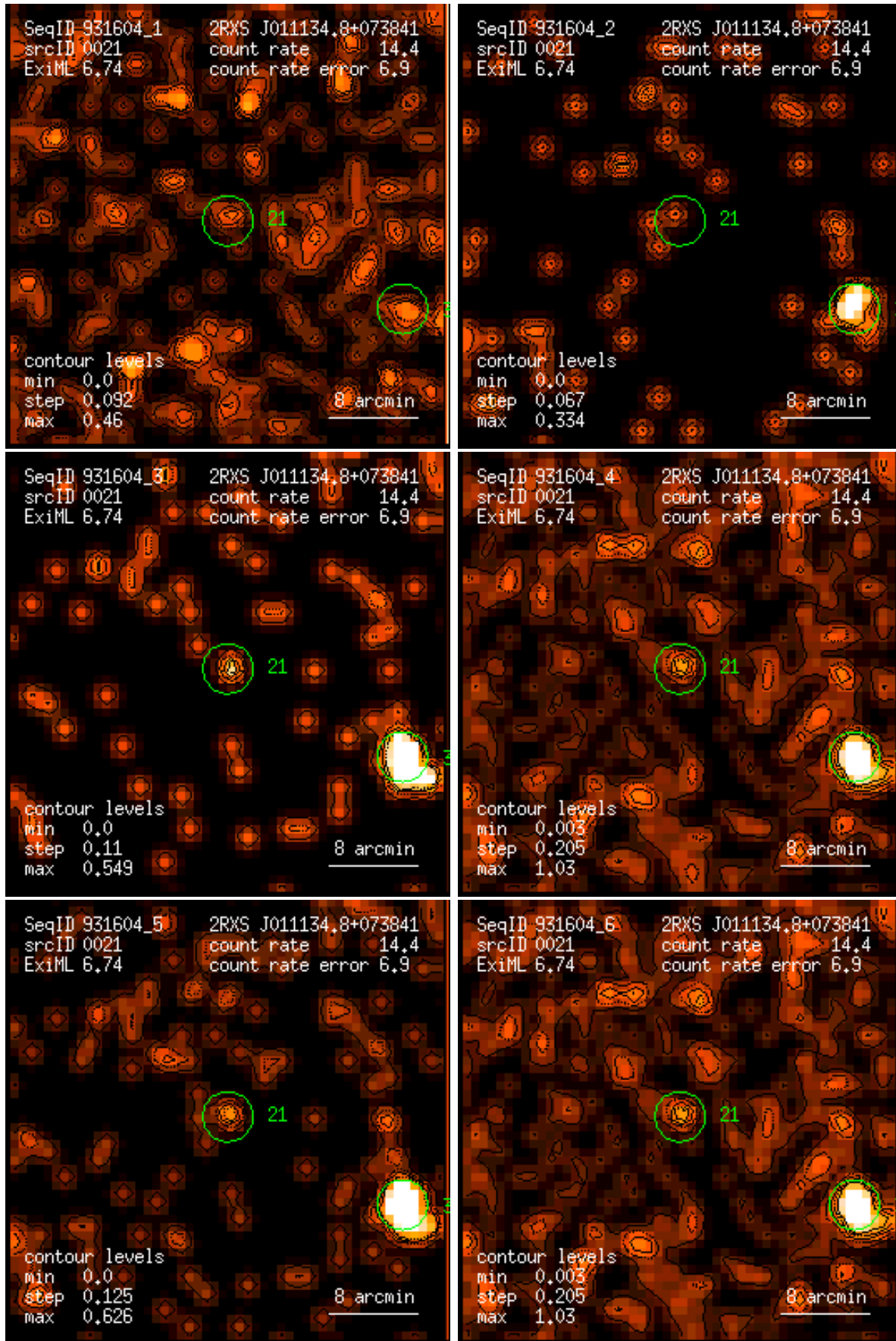
Figure 21: RASS 931604: detection 0021: band rate images, Gaussian filter: (1) PSPC channels 11 – 41, (2) 52 – 90, (3) 91 – 201, (4) 11 – 235, (5) 52 – 201, (6) 11 – 201. Broad band rates in counts/ks. Band rate contour levels in counts/ks/arcmin 2 .
