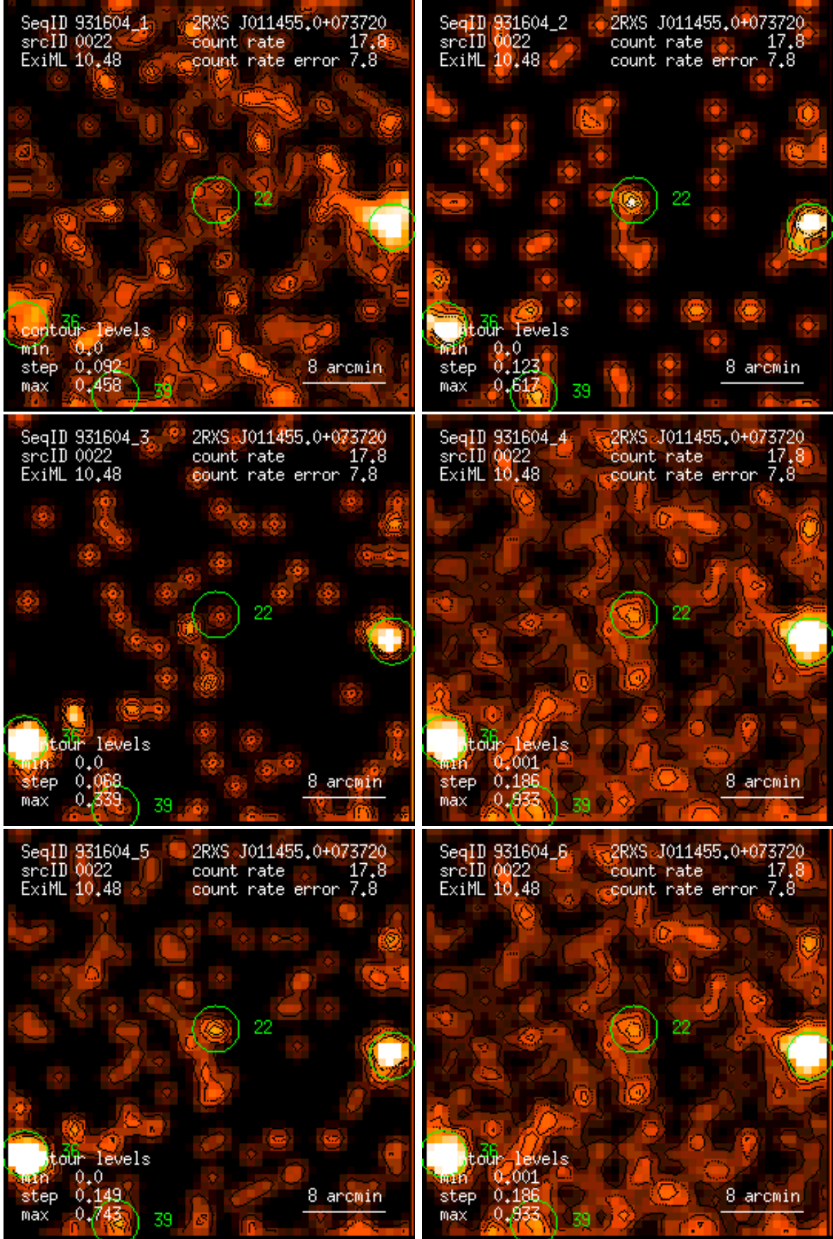
Figure 22: RASS 931604: detection 0022: band rate images, Gaussian filter: (1) PSPC channels 11 – 41, (2) 52 – 90, (3) 91 – 201, (4) 11 – 235, (5) 52 – 201, (6) 11 – 201. Broad band rates in counts/ks. Band rate contour levels in counts/ks/arcmin 2 .
