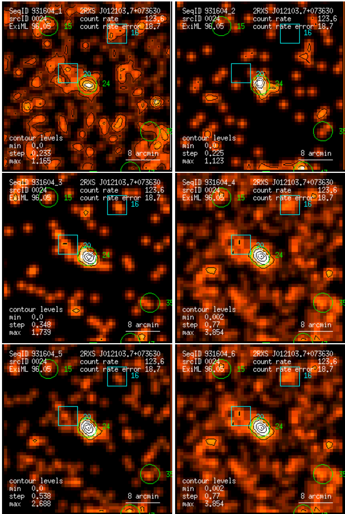
Figure 24: RASS 931604: detection 0024: band rate images, Gaussian filter: (1) PSPC channels 11 – 41, (2) 52 – 90, (3) 91 – 201, (4) 11 – 235, (5) 52 – 201, (6) 11 – 201. Broad band rates in counts/ks. Band rate contour levels in counts/ks/arcmin 2 .
