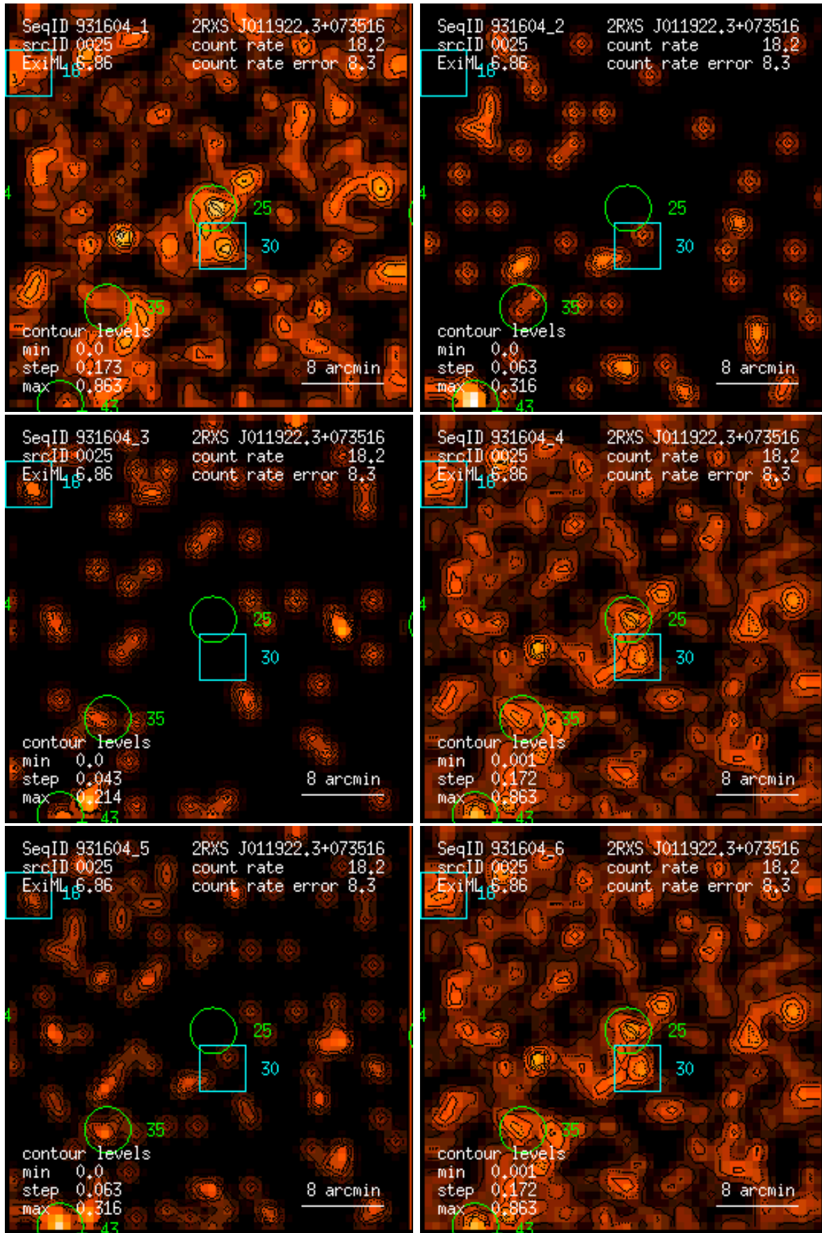
Figure 25: RASS 931604: detection 0025: band rate images, Gaussian filter: (1) PSPC channels 11 – 41, (2) 52 – 90, (3) 91 – 201, (4) 11 – 235, (5) 52 – 201, (6) 11 – 201. Broad band rates in counts/ks. Band rate contour levels in counts/ks/arcmin 2 .
