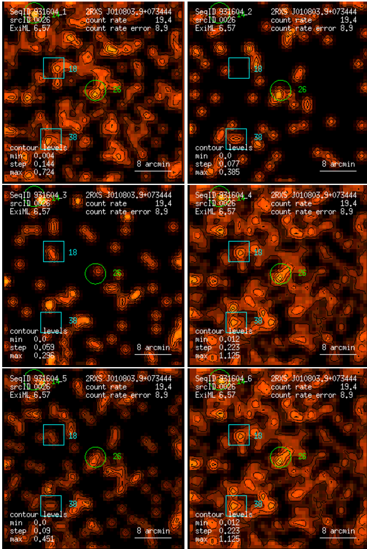
Figure 26: RASS 931604: detection 0026: band rate images, Gaussian filter: (1) PSPC channels 11 – 41, (2) 52 – 90, (3) 91 – 201, (4) 11 – 235, (5) 52 – 201, (6) 11 – 201. Broad band rates in counts/ks. Band rate contour levels in counts/ks/arcmin 2 .
