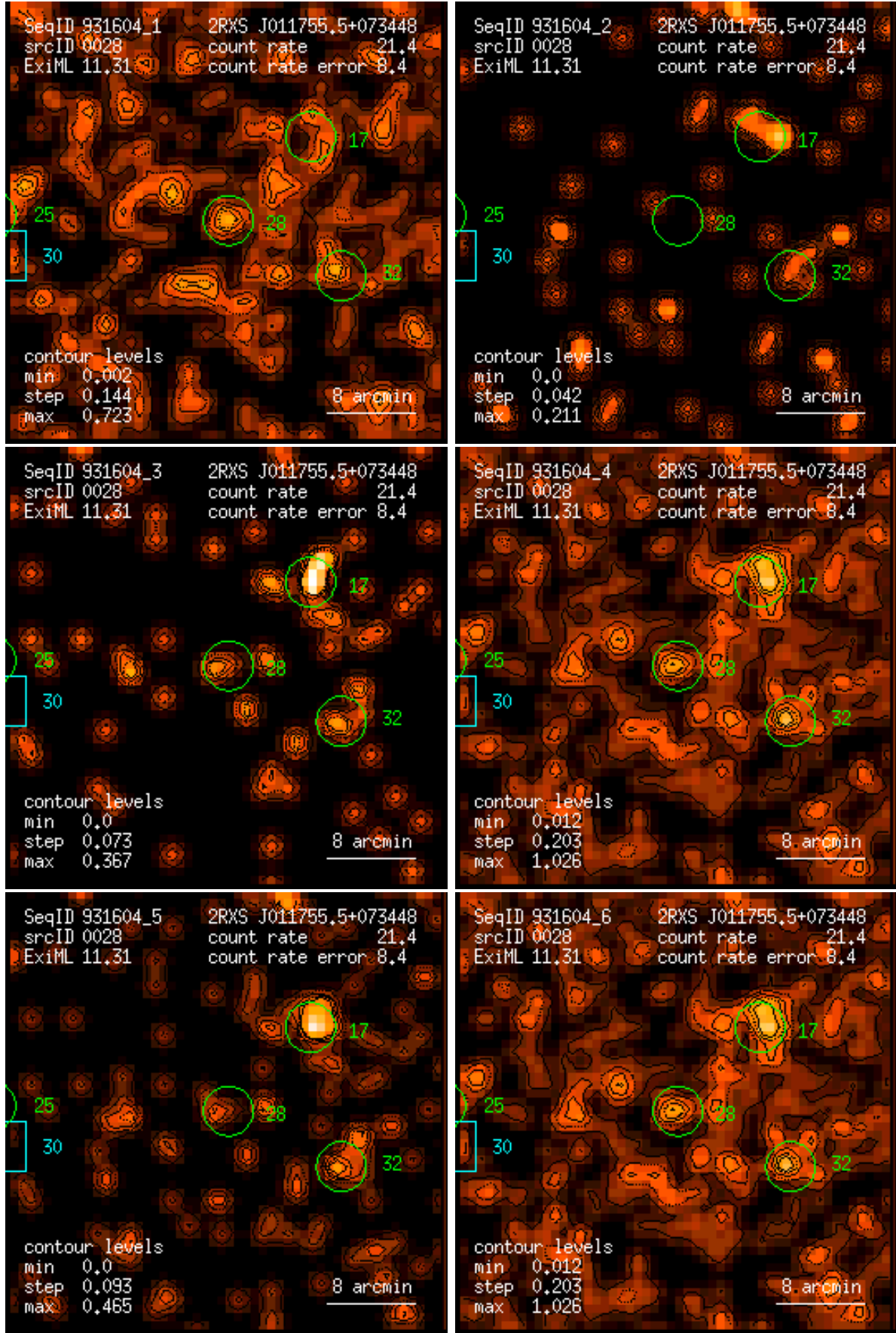
Figure 28: RASS 931604: detection 0028: band rate images, Gaussian filter: (1) PSPC channels 11 – 41, (2) 52 – 90, (3) 91 – 201, (4) 11 – 235, (5) 52 – 201, (6) 11 – 201. Broad band rates in counts/ks. Band rate contour levels in counts/ks/arcmin 2 .
