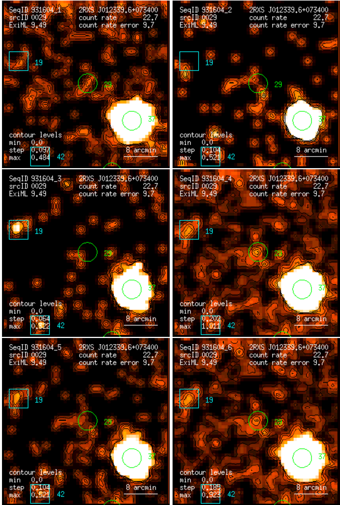
Figure 29: RASS 931604: detection 0029: band rate images, Gaussian filter: (1) PSPC channels 11 – 41, (2) 52 – 90, (3) 91 – 201, (4) 11 – 235, (5) 52 – 201, (6) 11 – 201. Broad band rates in counts/ks. Band rate contour levels in counts/ks/arcmin 2 .
