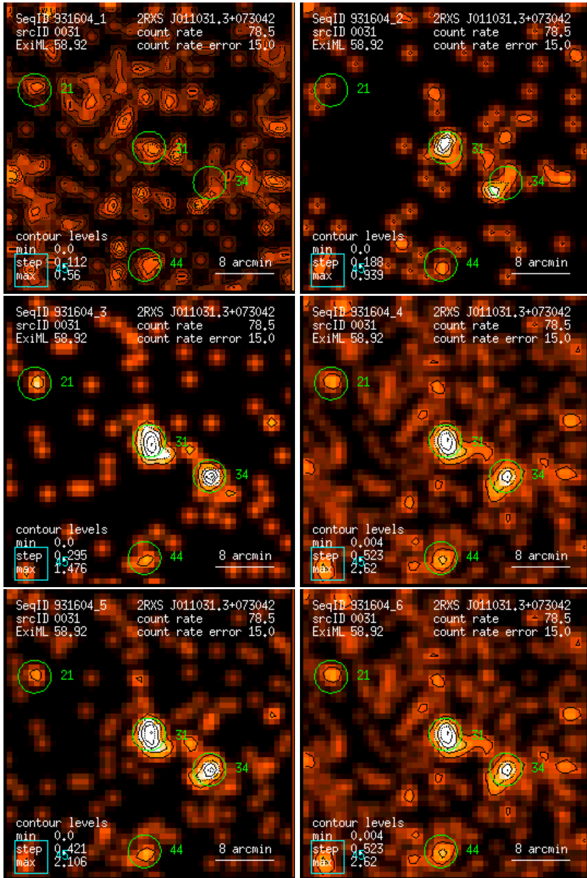
Figure 31: RASS 931604: detection 0031: band rate images, Gaussian filter: (1) PSPC channels 11 – 41, (2) 52 – 90, (3) 91 – 201, (4) 11 – 235, (5) 52 – 201, (6) 11 – 201. Broad band rates in counts/ks. Band rate contour levels in counts/ks/arcmin 2 .
