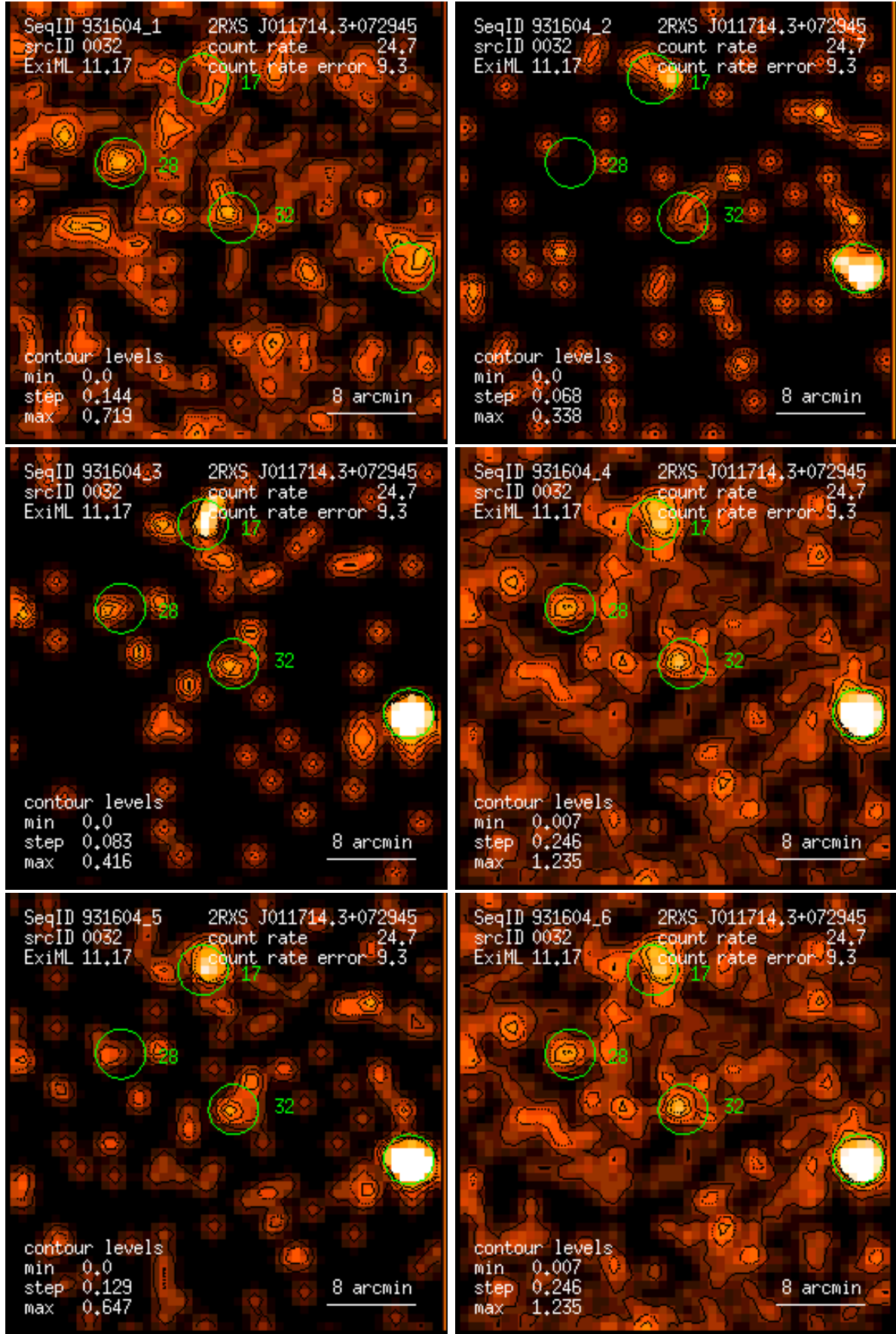
Figure 32: RASS 931604: detection 0032: band rate images, Gaussian filter: (1) PSPC channels 11 – 41, (2) 52 – 90, (3) 91 – 201, (4) 11 – 235, (5) 52 – 201, (6) 11 – 201. Broad band rates in counts/ks. Band rate contour levels in counts/ks/arcmin 2 .
