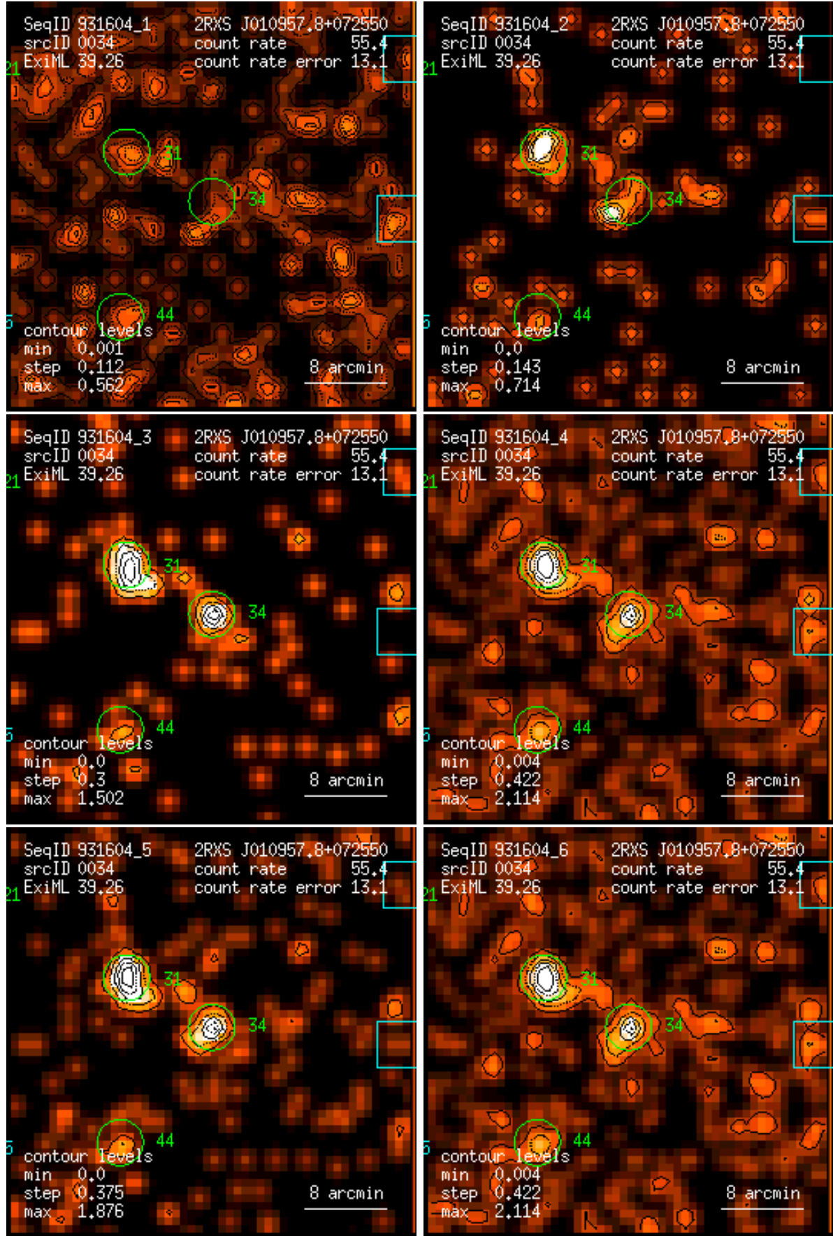
Figure 34: RASS 931604: detection 0034: band rate images, Gaussian filter: (1) PSPC channels 11 – 41, (2) 52 – 90, (3) 91 – 201, (4) 11 – 235, (5) 52 – 201, (6) 11 – 201. Broad band rates in counts/ks. Band rate contour levels in counts/ks/arcmin 2 .
