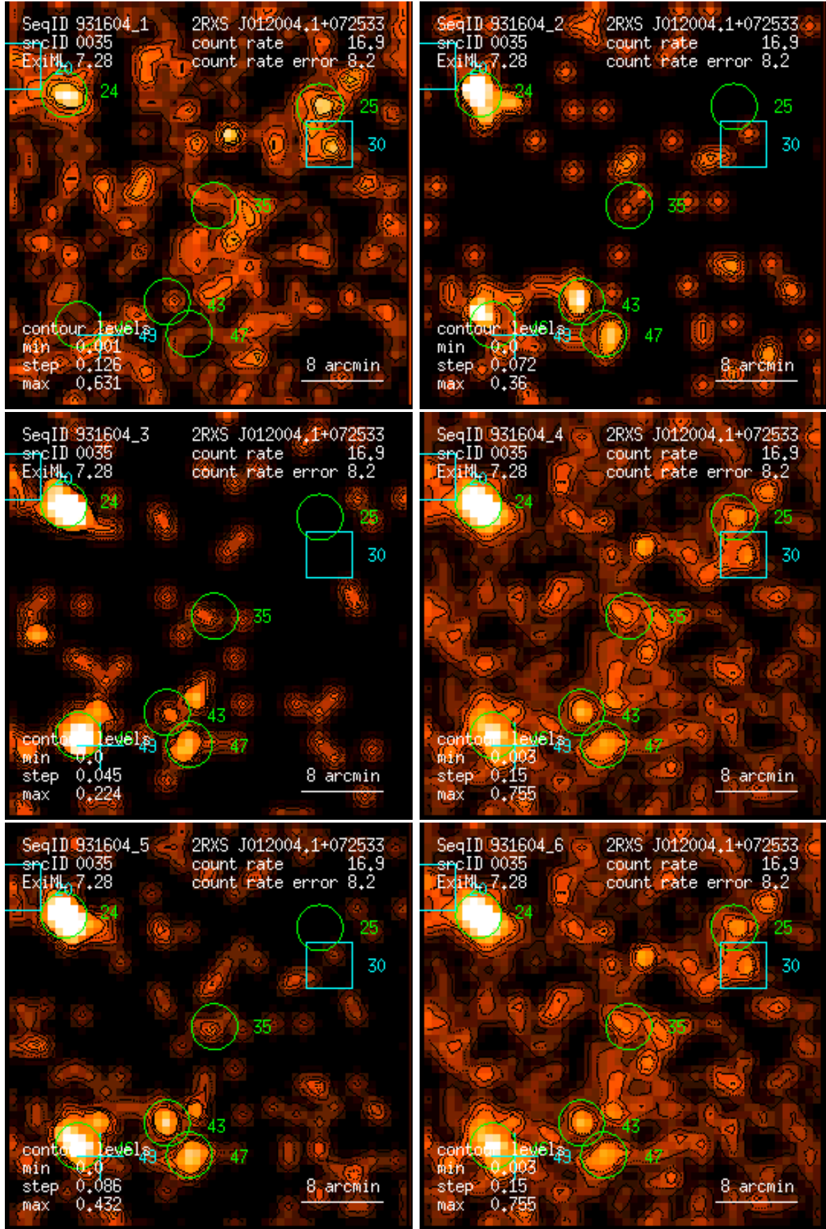
Figure 35: RASS 931604: detection 0035: band rate images, Gaussian filter: (1) PSPC channels 11 – 41, (2) 52 – 90, (3) 91 – 201, (4) 11 – 235, (5) 52 – 201, (6) 11 – 201. Broad band rates in counts/ks. Band rate contour levels in counts/ks/arcmin 2 .
