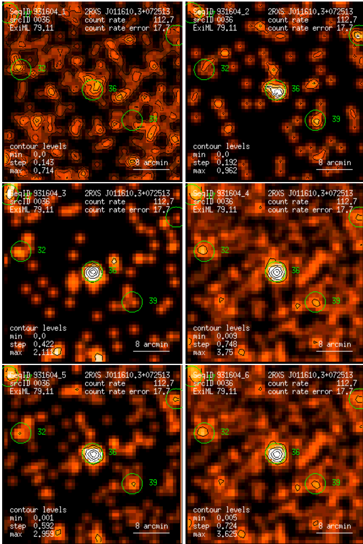
Figure 36: RASS 931604: detection 0036: band rate images, Gaussian filter: (1) PSPC channels 11 – 41, (2) 52 – 90, (3) 91 – 201, (4) 11 – 235, (5) 52 – 201, (6) 11 – 201. Broad band rates in counts/ks. Band rate contour levels in counts/ks/arcmin 2 .
