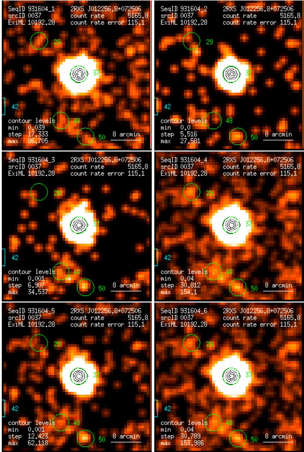
Figure 37: RASS 931604: detection 0037: band rate images, Gaussian filter: (1) PSPC channels 11 – 41, (2) 52 – 90, (3) 91 – 201, (4) 11 – 235, (5) 52 – 201, (6) 11 – 201. Broad band rates in counts/ks. Band rate contour levels in counts/ks/arcmin 2 .
