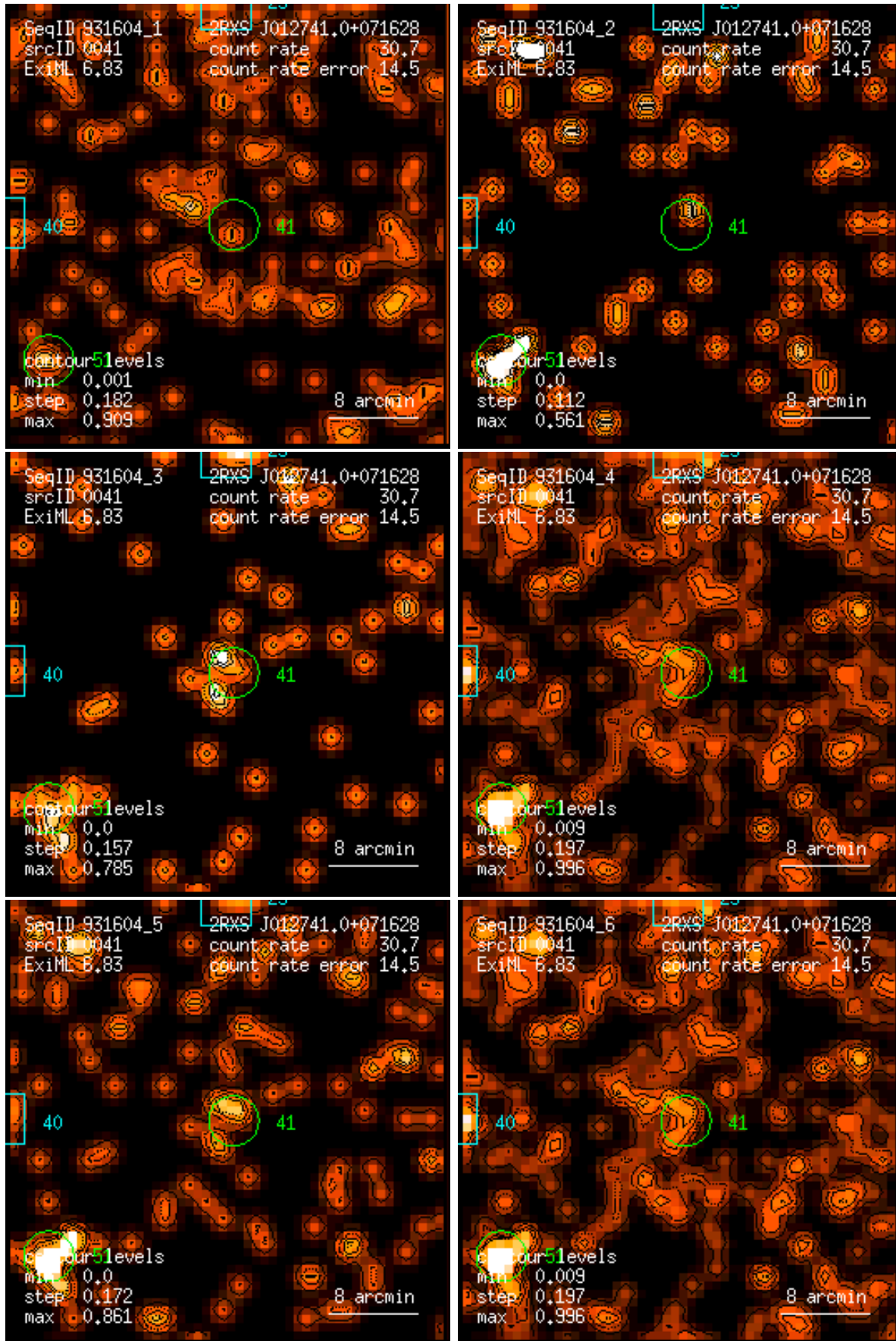
Figure 41: RASS 931604: detection 0041: band rate images, Gaussian filter: (1) PSPC channels 11 – 41, (2) 52 – 90, (3) 91 – 201, (4) 11 – 235, (5) 52 – 201, (6) 11 – 201. Broad band rates in counts/ks. Band rate contour levels in counts/ks/arcmin 2 .
