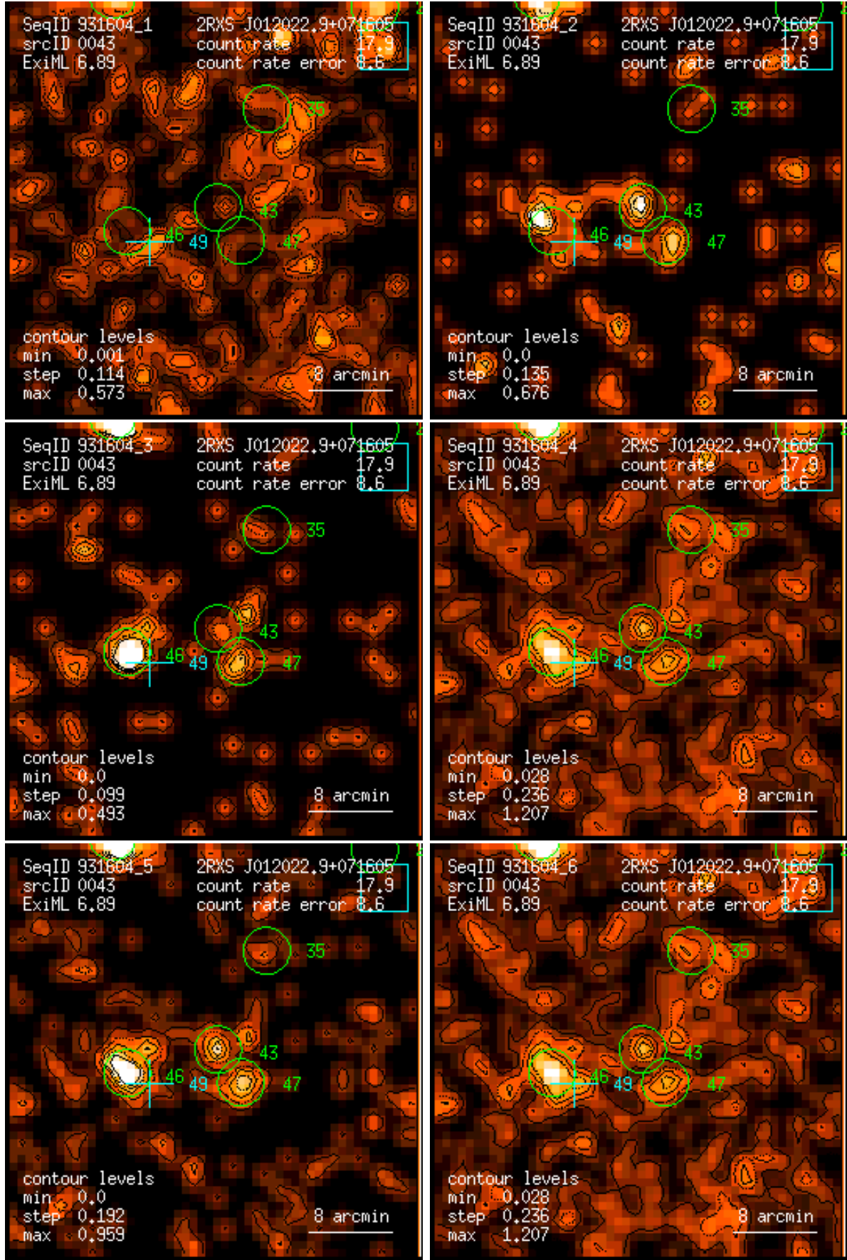
Figure 43: RASS 931604: detection 0043: band rate images, Gaussian filter: (1) PSPC channels 11 – 41, (2) 52 – 90, (3) 91 – 201, (4) 11 – 235, (5) 52 – 201, (6) 11 – 201. Broad band rates in counts/ks. Band rate contour levels in counts/ks/arcmin 2 .
