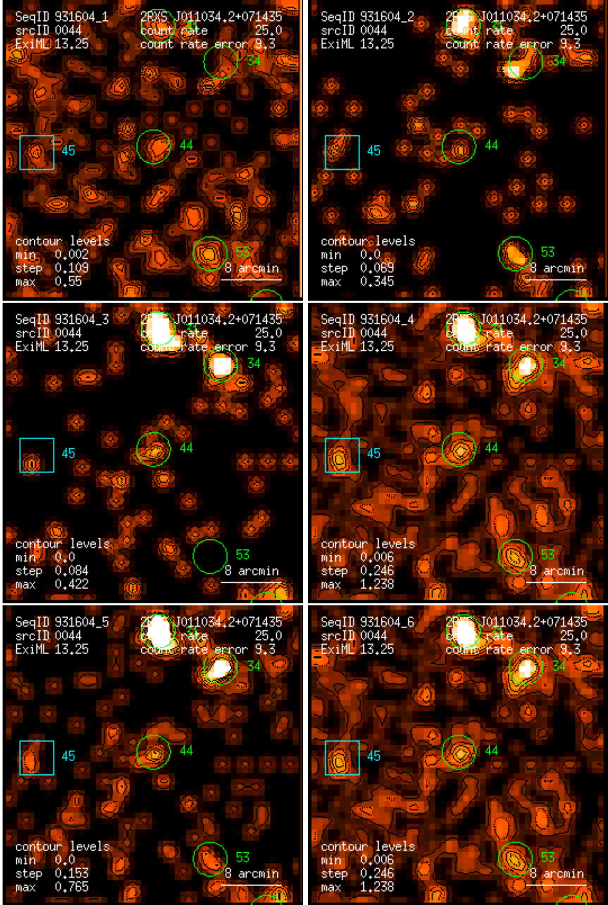
Figure 44: RASS 931604: detection 0044: band rate images, Gaussian filter: (1) PSPC channels 11 – 41, (2) 52 – 90, (3) 91 – 201, (4) 11 – 235, (5) 52 – 201, (6) 11 – 201. Broad band rates in counts/ks. Band rate contour levels in counts/ks/arcmin 2 .
