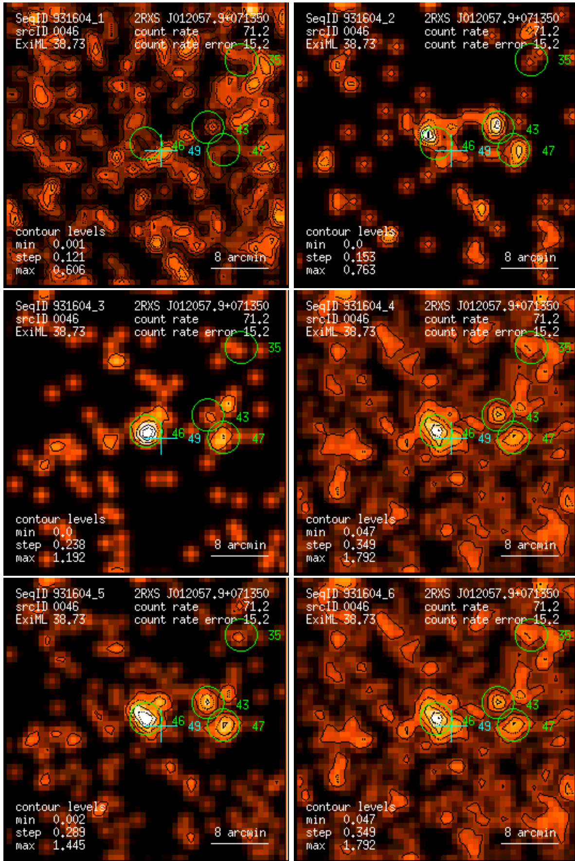
Figure 46: RASS 931604: detection 0046: band rate images, Gaussian filter: (1) PSPC channels 11 – 41, (2) 52 – 90, (3) 91 – 201, (4) 11 – 235, (5) 52 – 201, (6) 11 – 201. Broad band rates in counts/ks. Band rate contour levels in counts/ks/arcmin 2 .
