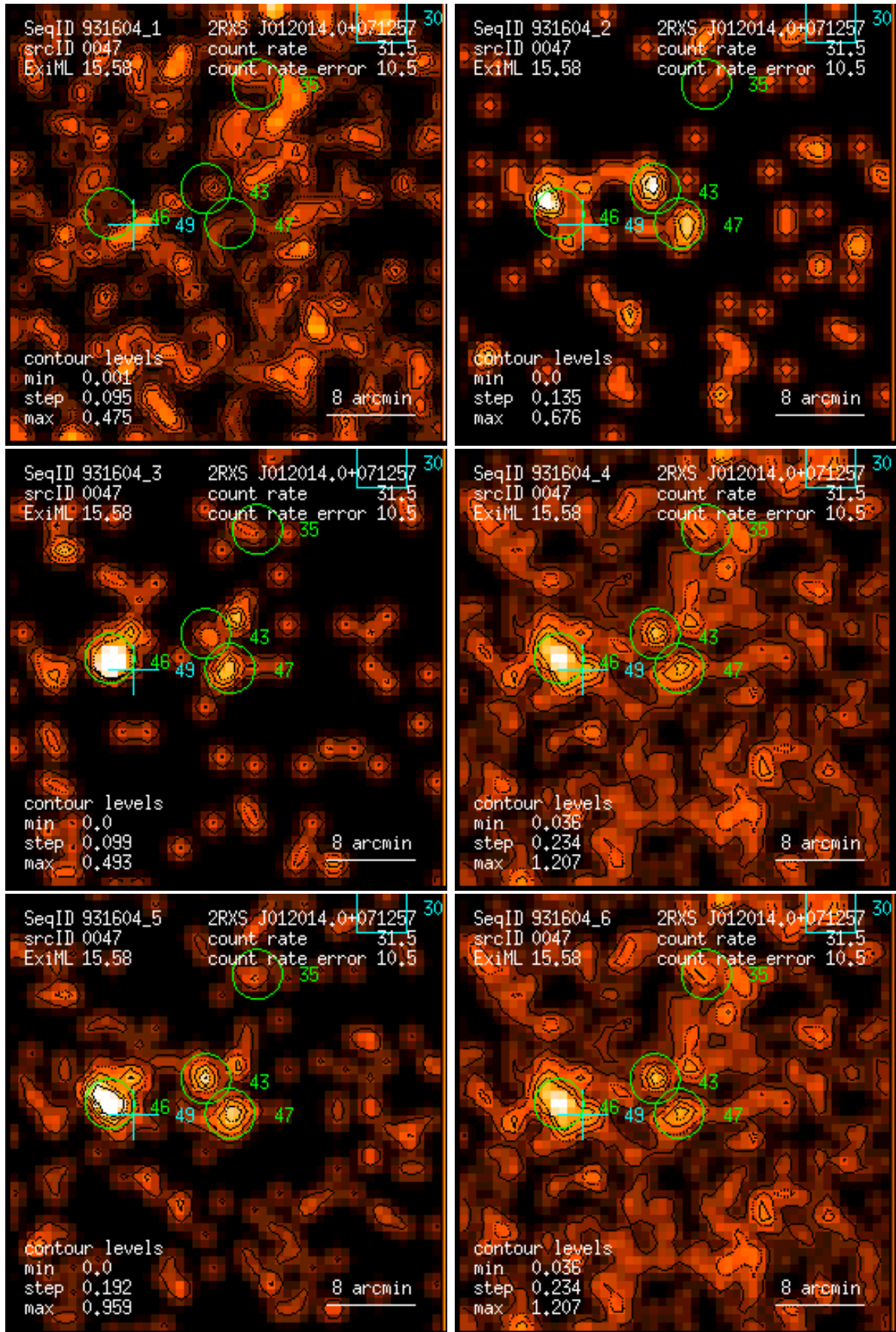
Figure 47: RASS 931604: detection 0047: band rate images, Gaussian filter: (1) PSPC channels 11 – 41, (2) 52 – 90, (3) 91 – 201, (4) 11 – 235, (5) 52 – 201, (6) 11 – 201. Broad band rates in counts/ks. Band rate contour levels in counts/ks/arcmin 2 .
