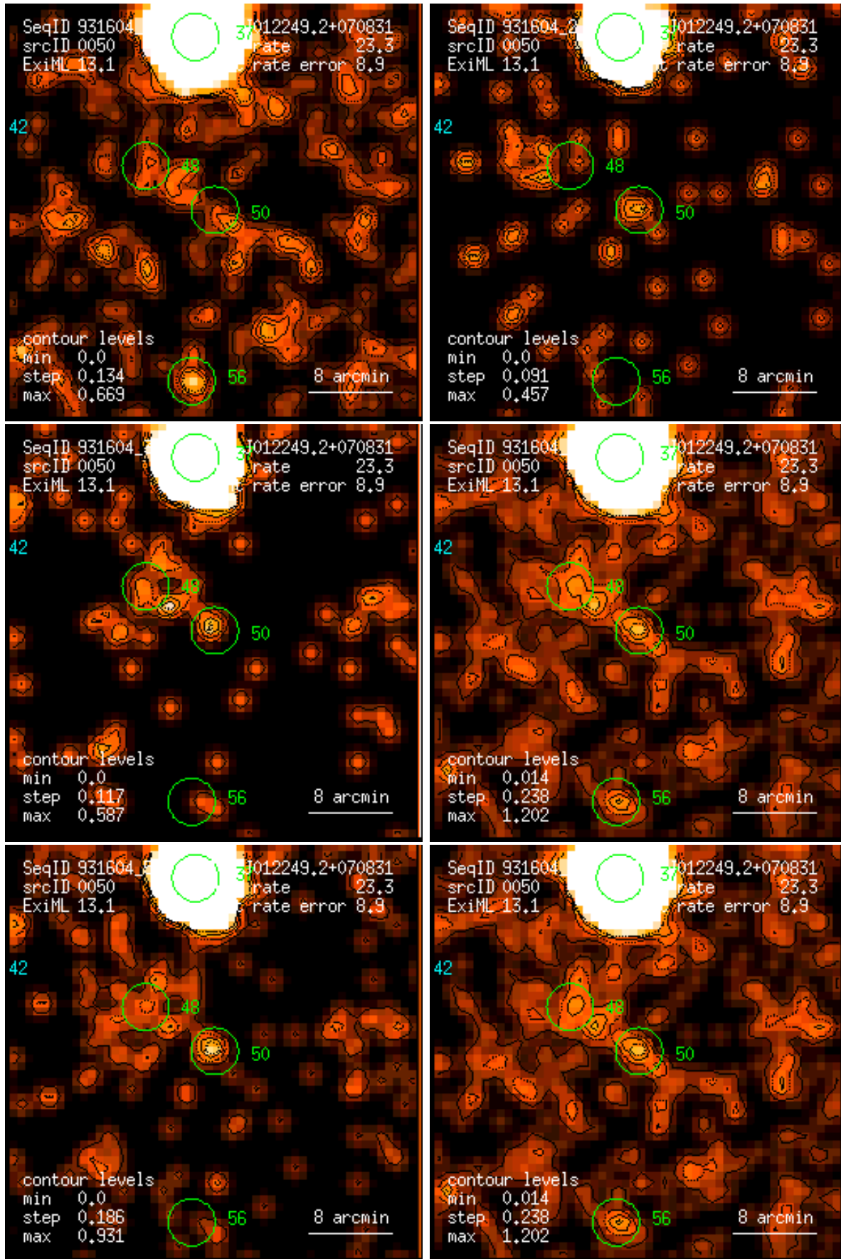
Figure 50: RASS 931604: detection 0050: band rate images, Gaussian filter: (1) PSPC channels 11 – 41, (2) 52 – 90, (3) 91 – 201, (4) 11 – 235, (5) 52 – 201, (6) 11 – 201. Broad band rates in counts/ks. Band rate contour levels in counts/ks/arcmin 2 .
