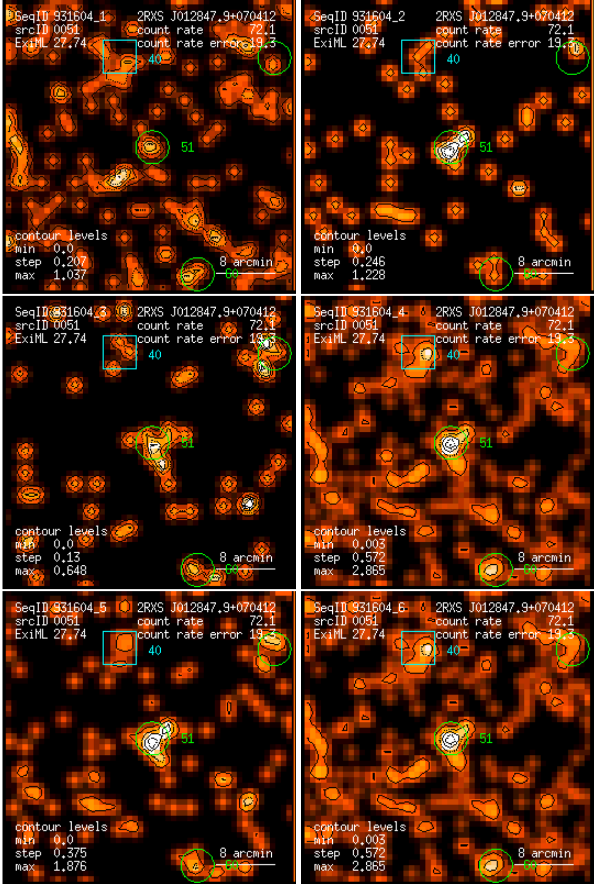
Figure 51: RASS 931604: detection 0051: band rate images, Gaussian filter: (1) PSPC channels 11 – 41, (2) 52 – 90, (3) 91 – 201, (4) 11 – 235, (5) 52 – 201, (6) 11 – 201. Broad band rates in counts/ks. Band rate contour levels in counts/ks/arcmin 2 .
