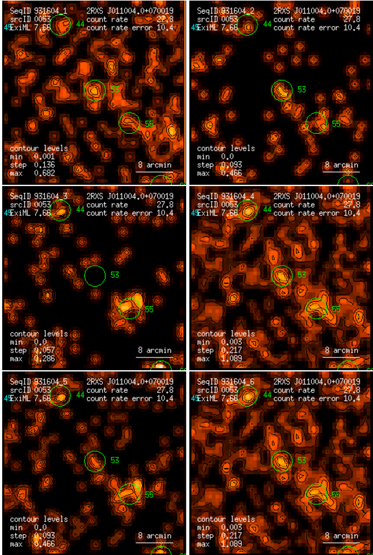
Figure 53: RASS 931604: detection 0053: band rate images, Gaussian filter: (1) PSPC channels 11 – 41, (2) 52 – 90, (3) 91 – 201, (4) 11 – 235, (5) 52 – 201, (6) 11 – 201. Broad band rates in counts/ks. Band rate contour levels in counts/ks/arcmin 2 .
