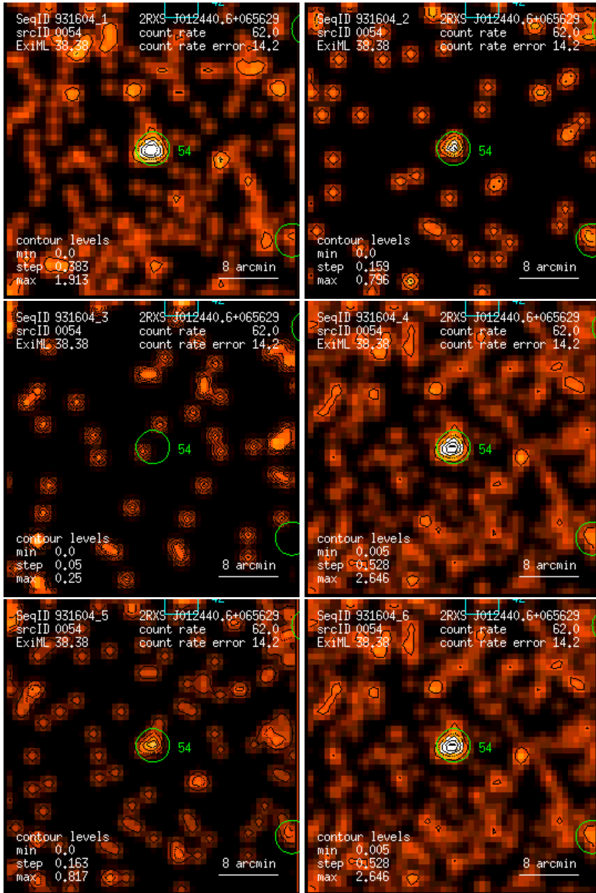
Figure 54: RASS 931604: detection 0054: band rate images, Gaussian filter: (1) PSPC channels 11 – 41, (2) 52 – 90, (3) 91 – 201, (4) 11 – 235, (5) 52 – 201, (6) 11 – 201. Broad band rates in counts/ks. Band rate contour levels in counts/ks/arcmin 2 .
