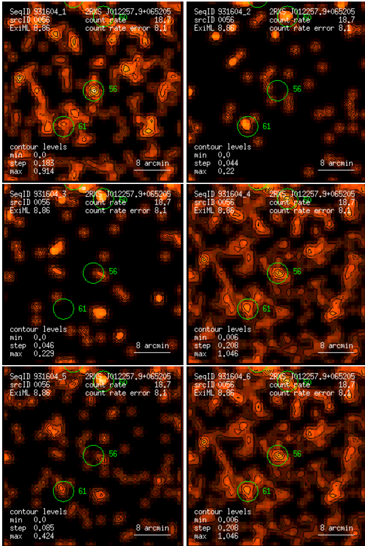
Figure 56: RASS 931604: detection 0056: band rate images, Gaussian filter: (1) PSPC channels 11 – 41, (2) 52 – 90, (3) 91 – 201, (4) 11 – 235, (5) 52 – 201, (6) 11 – 201. Broad band rates in counts/ks. Band rate contour levels in counts/ks/arcmin 2 .
