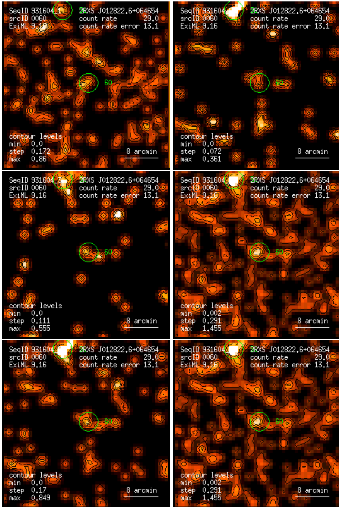
Figure 60: RASS 931604: detection 0060: band rate images, Gaussian filter: (1) PSPC channels 11 – 41, (2) 52 – 90, (3) 91 – 201, (4) 11 – 235, (5) 52 – 201, (6) 11 – 201. Broad band rates in counts/ks. Band rate contour levels in counts/ks/arcmin 2 .
