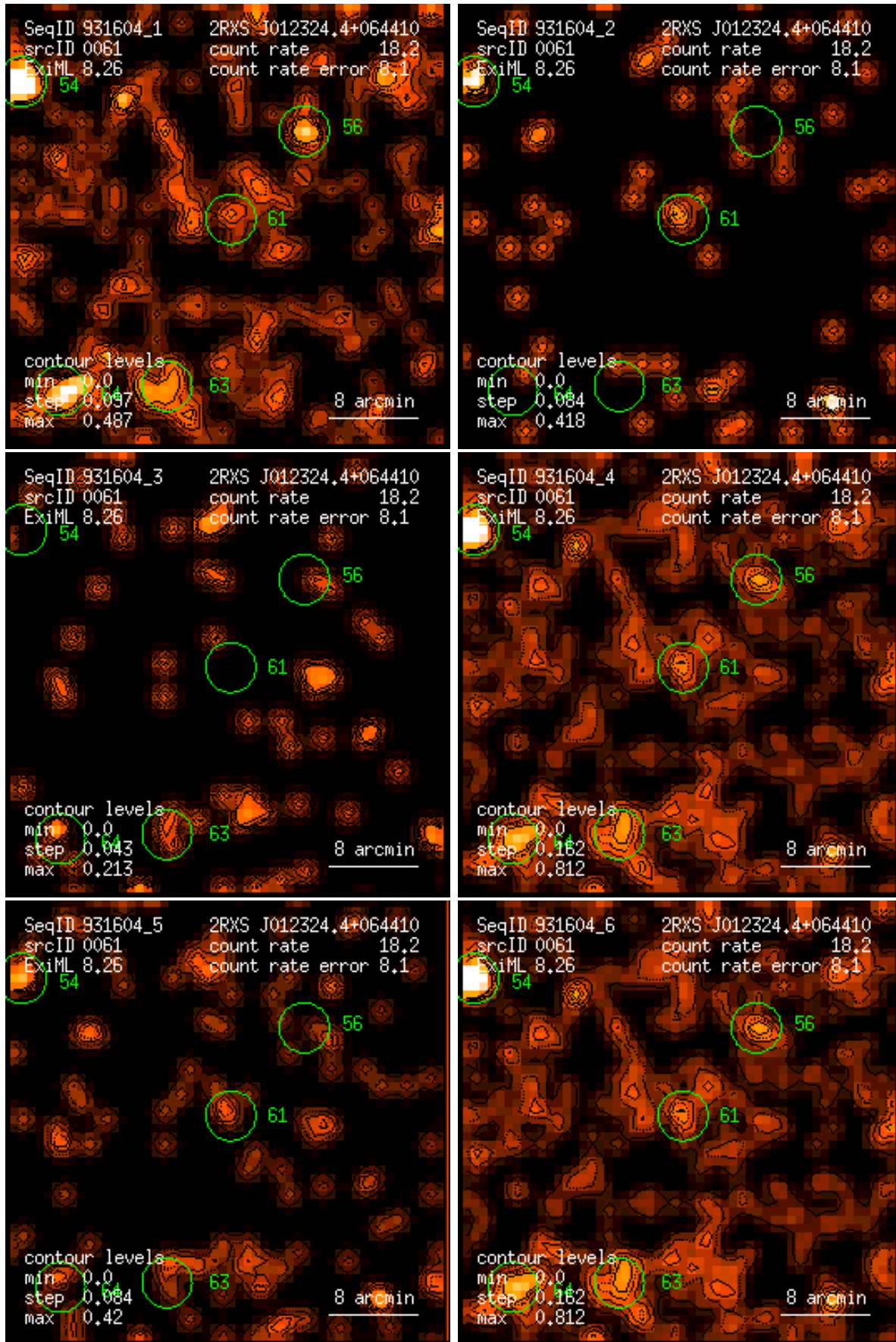
Figure 61: RASS 931604: detection 0061: band rate images, Gaussian filter: (1) PSPC channels 11 – 41, (2) 52 – 90, (3) 91 – 201, (4) 11 – 235, (5) 52 – 201, (6) 11 – 201. Broad band rates in counts/ks. Band rate contour levels in counts/ks/arcmin 2 .
