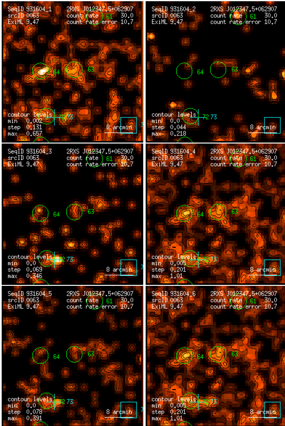
Figure 63: RASS 931604: detection 0063: band rate images, Gaussian filter: (1) PSPC channels 11 – 41, (2) 52 – 90, (3) 91 – 201, (4) 11 – 235, (5) 52 – 201, (6) 11 – 201. Broad band rates in counts/ks. Band rate contour levels in counts/ks/arcmin 2 .
