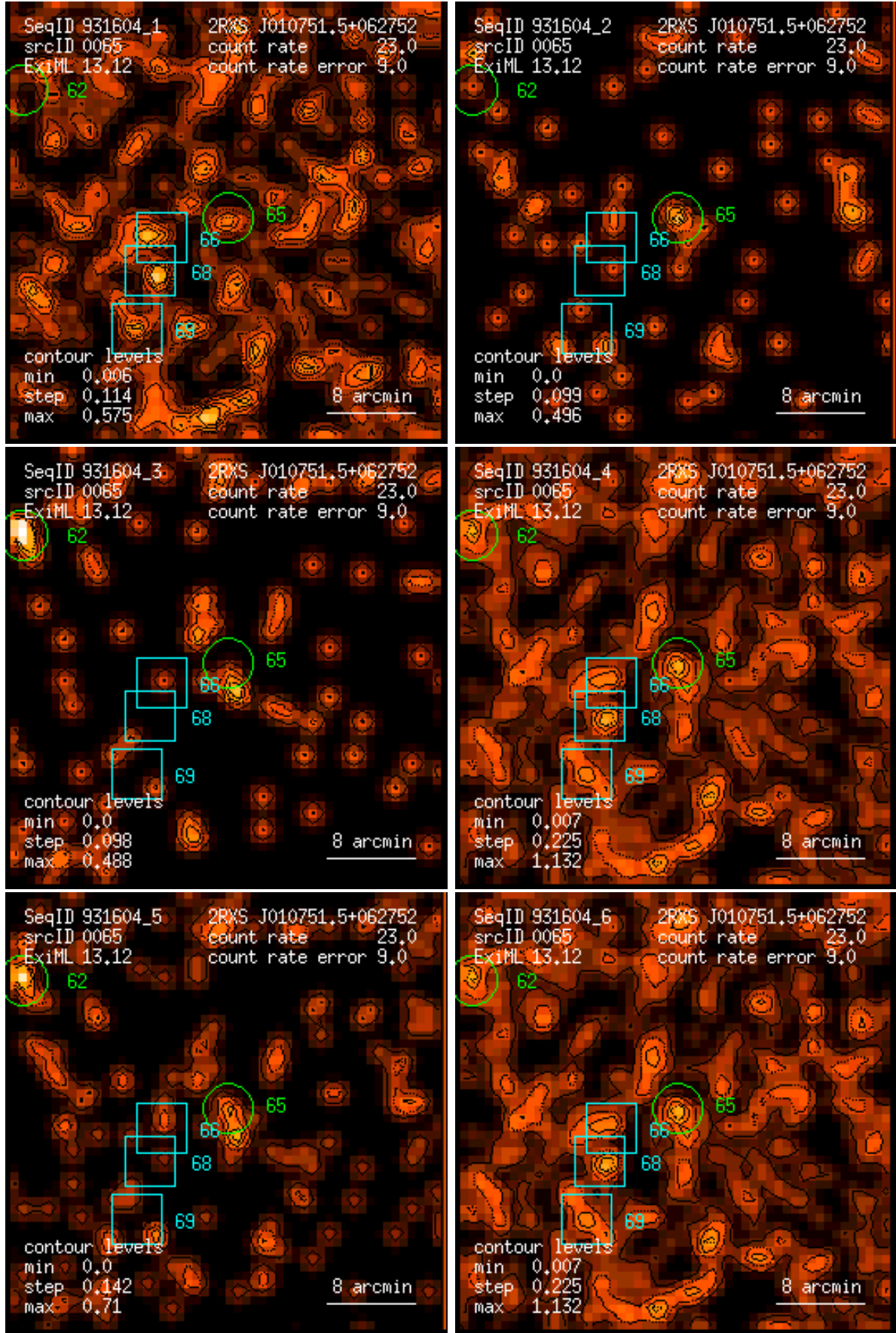
Figure 65: RASS 931604: detection 0065: band rate images, Gaussian filter: (1) PSPC channels 11 – 41, (2) 52 – 90, (3) 91 – 201, (4) 11 – 235, (5) 52 – 201, (6) 11 – 201. Broad band rates in counts/ks. Band rate contour levels in counts/ks/arcmin 2 .
