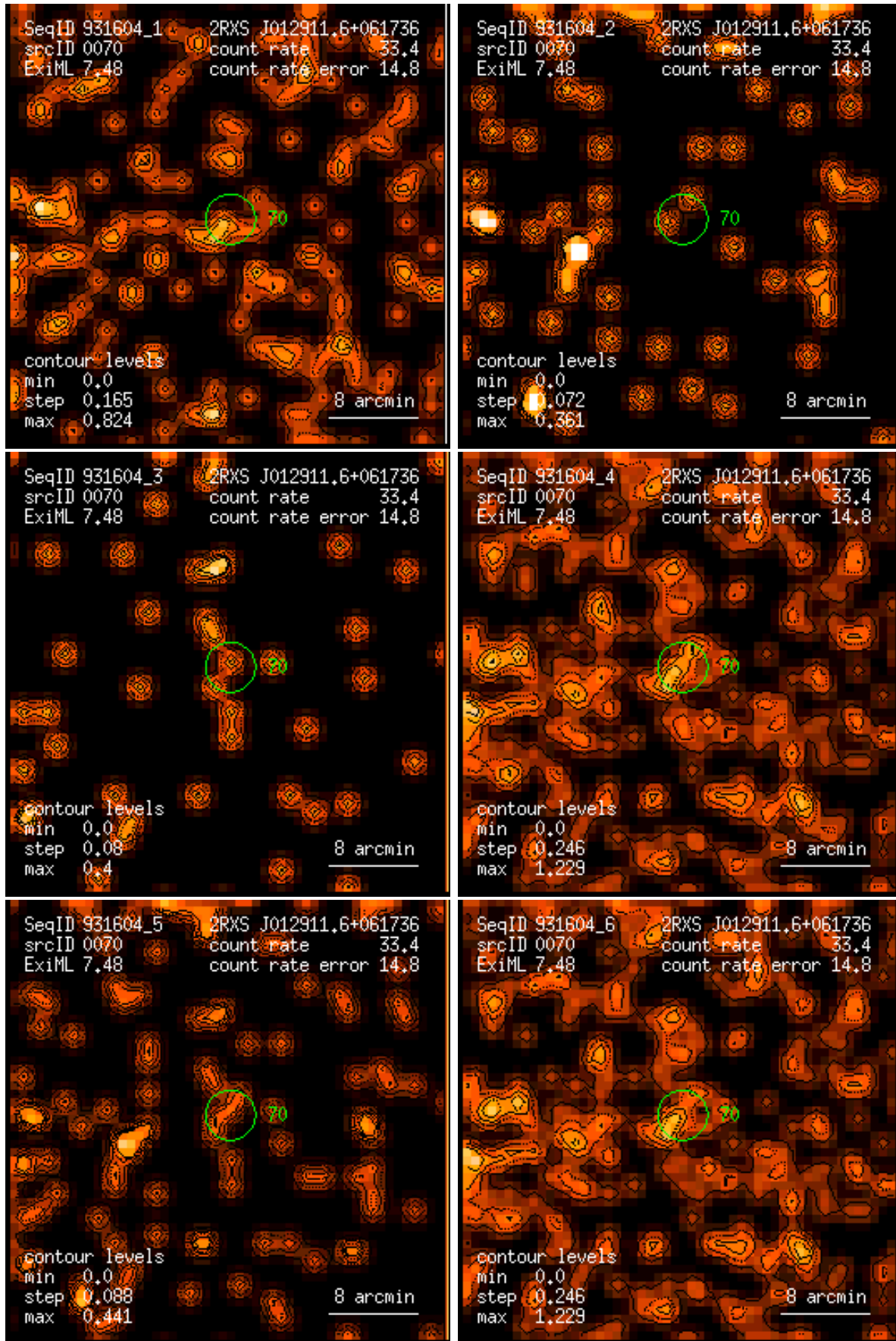
Figure 70: RASS 931604: detection 0070: band rate images, Gaussian filter: (1) PSPC channels 11 – 41, (2) 52 – 90, (3) 91 – 201, (4) 11 – 235, (5) 52 – 201, (6) 11 – 201. Broad band rates in counts/ks. Band rate contour levels in counts/ks/arcmin 2 .
