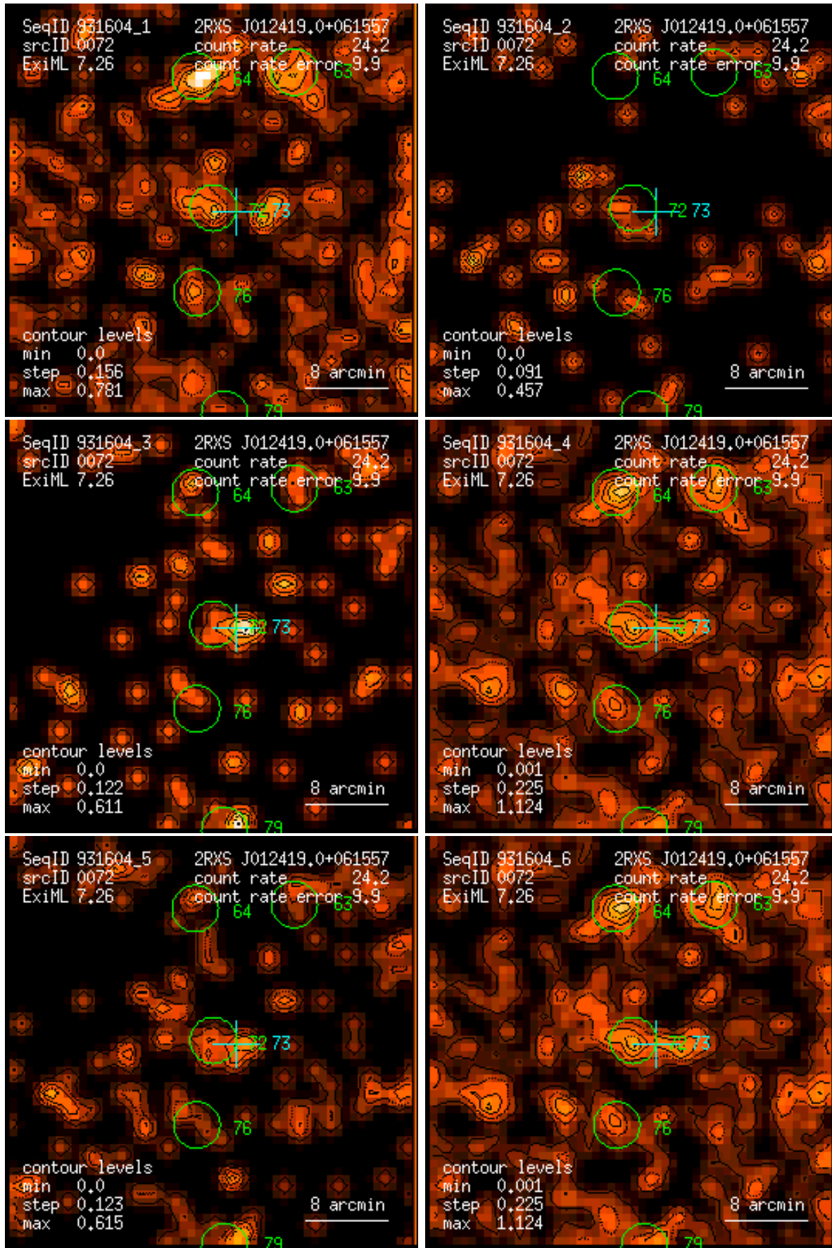
Figure 72: RASS 931604: detection 0072: band rate images, Gaussian filter: (1) PSPC channels 11 – 41, (2) 52 – 90, (3) 91 – 201, (4) 11 – 235, (5) 52 – 201, (6) 11 – 201. Broad band rates in counts/ks. Band rate contour levels in counts/ks/arcmin 2 .
