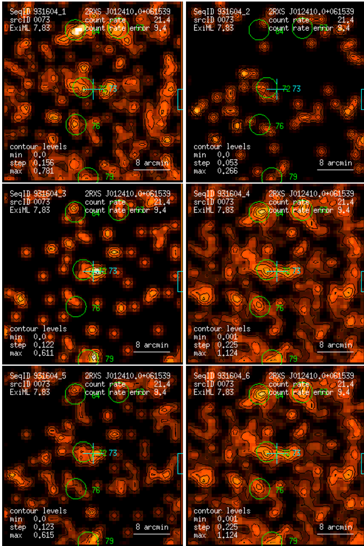
Figure 73: RASS 931604: detection 0073: band rate images, Gaussian filter: (1) PSPC channels 11 – 41, (2) 52 – 90, (3) 91 – 201, (4) 11 – 235, (5) 52 – 201, (6) 11 – 201. Broad band rates in counts/ks. Band rate contour levels in counts/ks/arcmin 2 .
