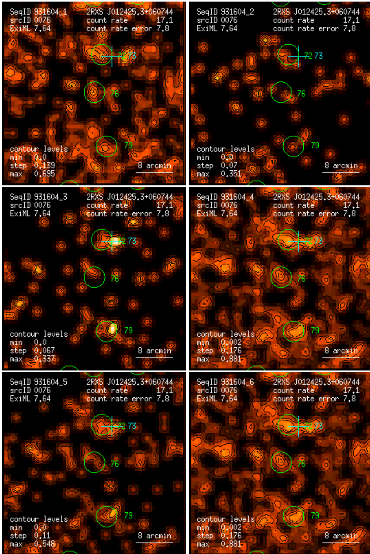
Figure 76: RASS 931604: detection 0076: band rate images, Gaussian filter: (1) PSPC channels 11 – 41, (2) 52 – 90, (3) 91 – 201, (4) 11 – 235, (5) 52 – 201, (6) 11 – 201. Broad band rates in counts/ks. Band rate contour levels in counts/ks/arcmin 2 .
