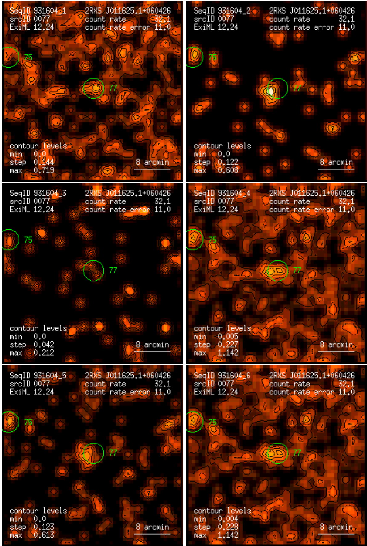
Figure 77: RASS 931604: detection 0077: band rate images, Gaussian filter: (1) PSPC channels 11 – 41, (2) 52 – 90, (3) 91 – 201, (4) 11 – 235, (5) 52 – 201, (6) 11 – 201. Broad band rates in counts/ks. Band rate contour levels in counts/ks/arcmin 2 .
