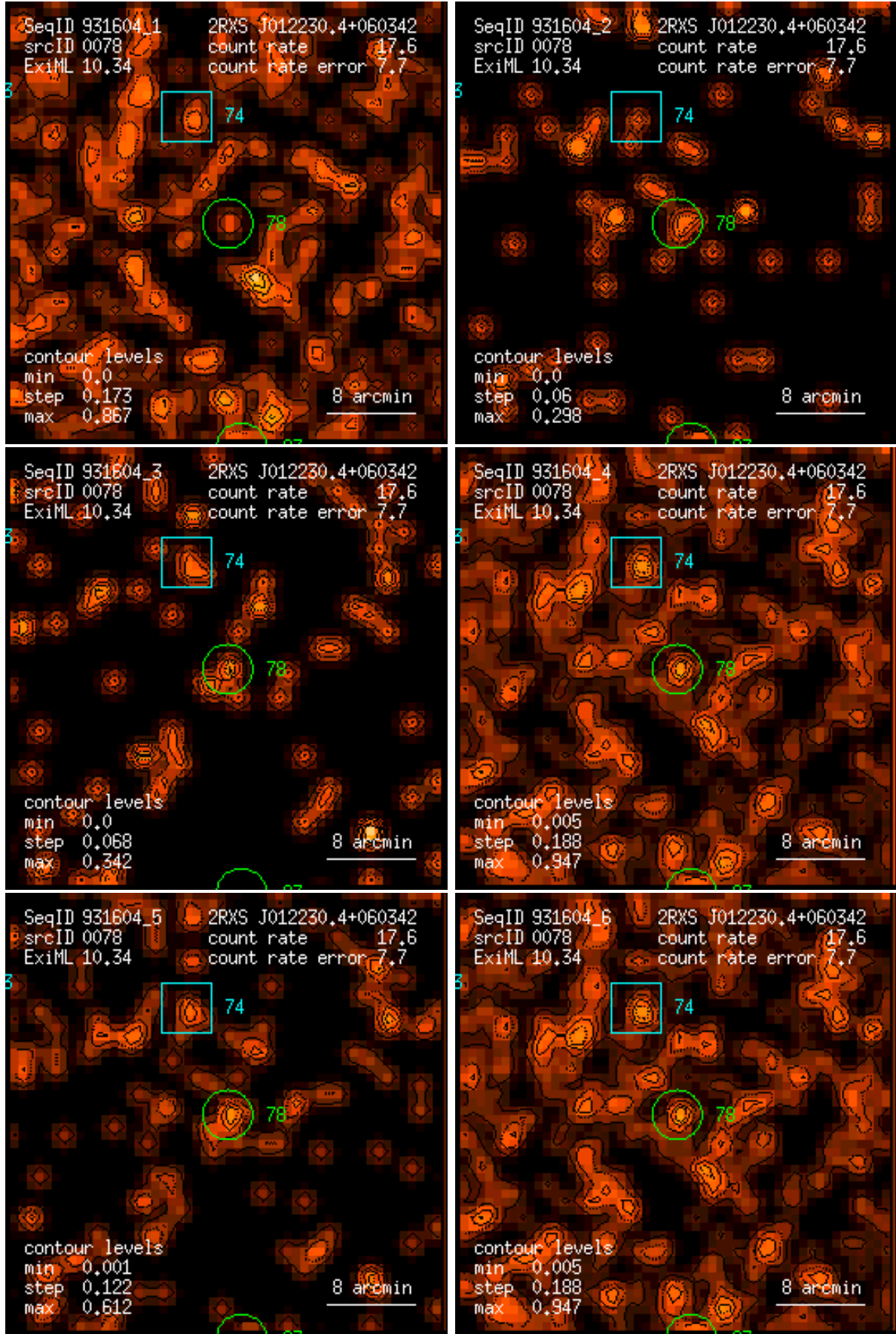
Figure 78: RASS 931604: detection 0078: band rate images, Gaussian filter: (1) PSPC channels 11 – 41, (2) 52 – 90, (3) 91 – 201, (4) 11 – 235, (5) 52 – 201, (6) 11 – 201. Broad band rates in counts/ks. Band rate contour levels in counts/ks/arcmin 2 .
