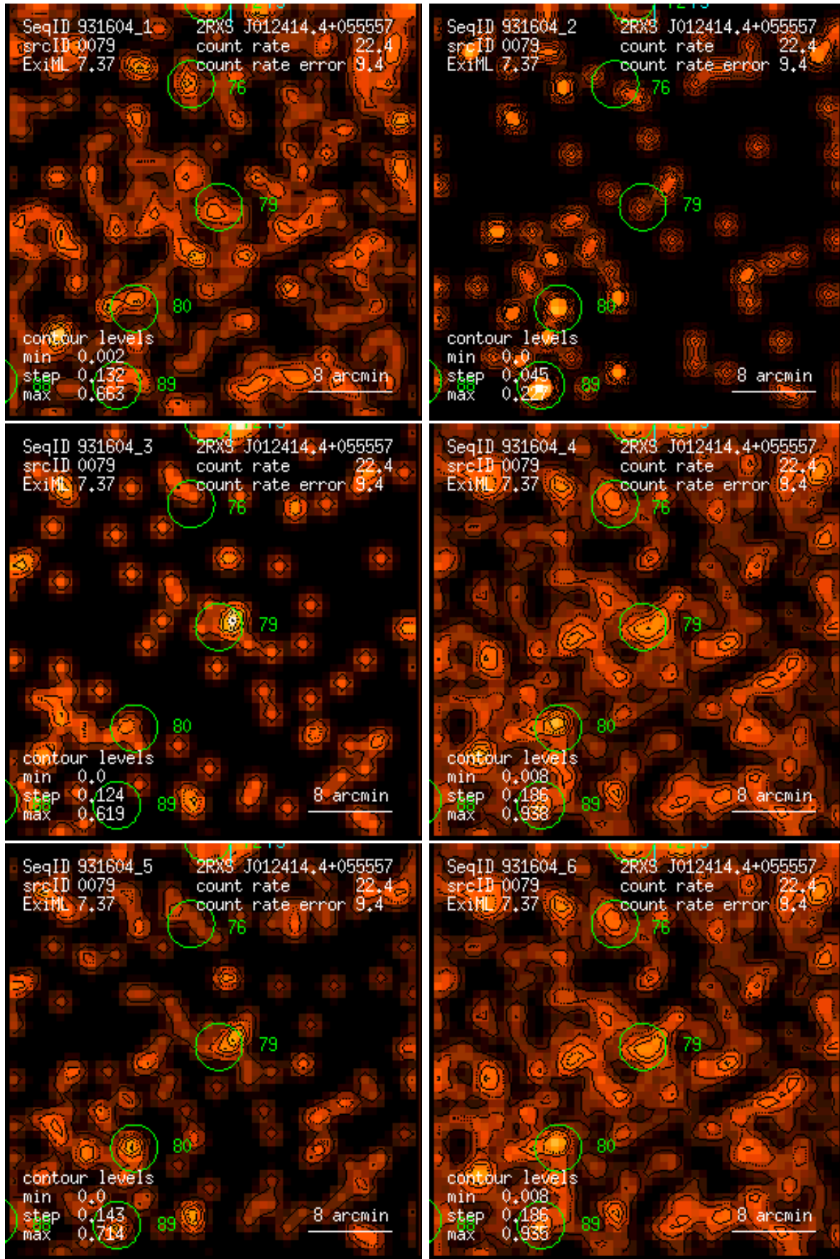
Figure 79: RASS 931604: detection 0079: band rate images, Gaussian filter: (1) PSPC channels 11 – 41, (2) 52 – 90, (3) 91 – 201, (4) 11 – 235, (5) 52 – 201, (6) 11 – 201. Broad band rates in counts/ks. Band rate contour levels in counts/ks/arcmin 2 .
